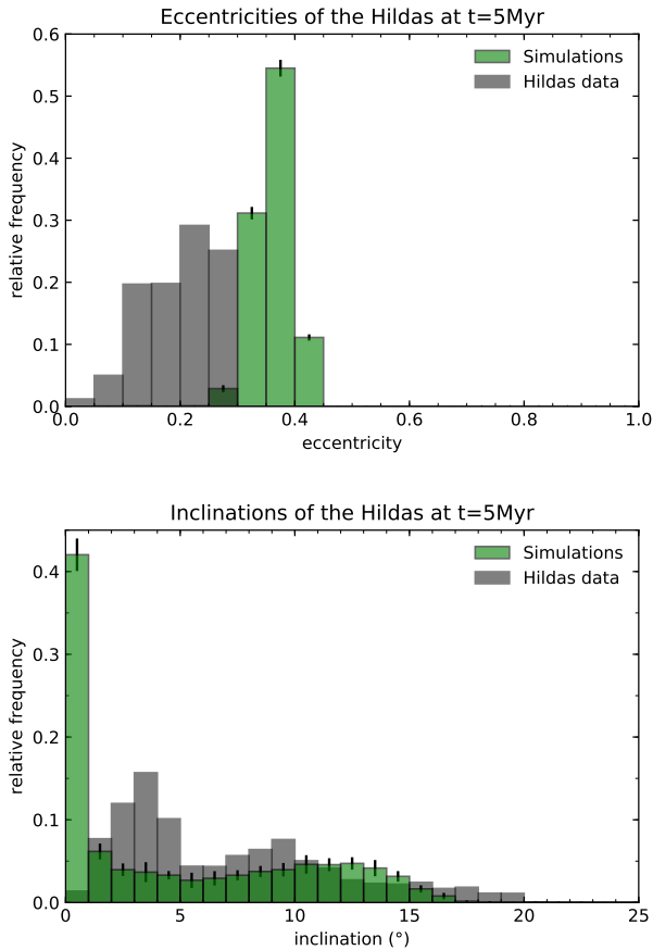
Fig. 15. Osculating eccentricities (top figure) and inclinations (bottom figure) of the Hilda asteroids at t = 5 Myr with Jupiter and Saturn that end locked in the 1:2 resonance.
