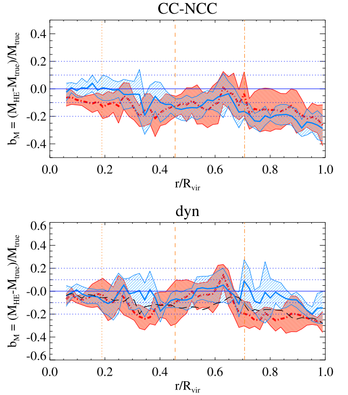
Figure 8. Median radial profile of the mass bias, as in Figure 5, distinguishing among different cluster populations. Upper panel: CC/NCC (blue solid/red dotted-dashed line); lower panel: regular/disturbed (blue solid/red dotted-dashed line) clusters; intermediate systems are marked by the thin black line and, for simplicity, no dispersion is marked. The hydrostatic mass, M_{\text{HE}} , is calculated using T_{\text{mw}} . Shaded areas represent the median absolute deviation from the median value, in each radial bin. From left to right, vertical lines mark median values of R_{2500} , R_{500} , and R_{200} , respectively.
