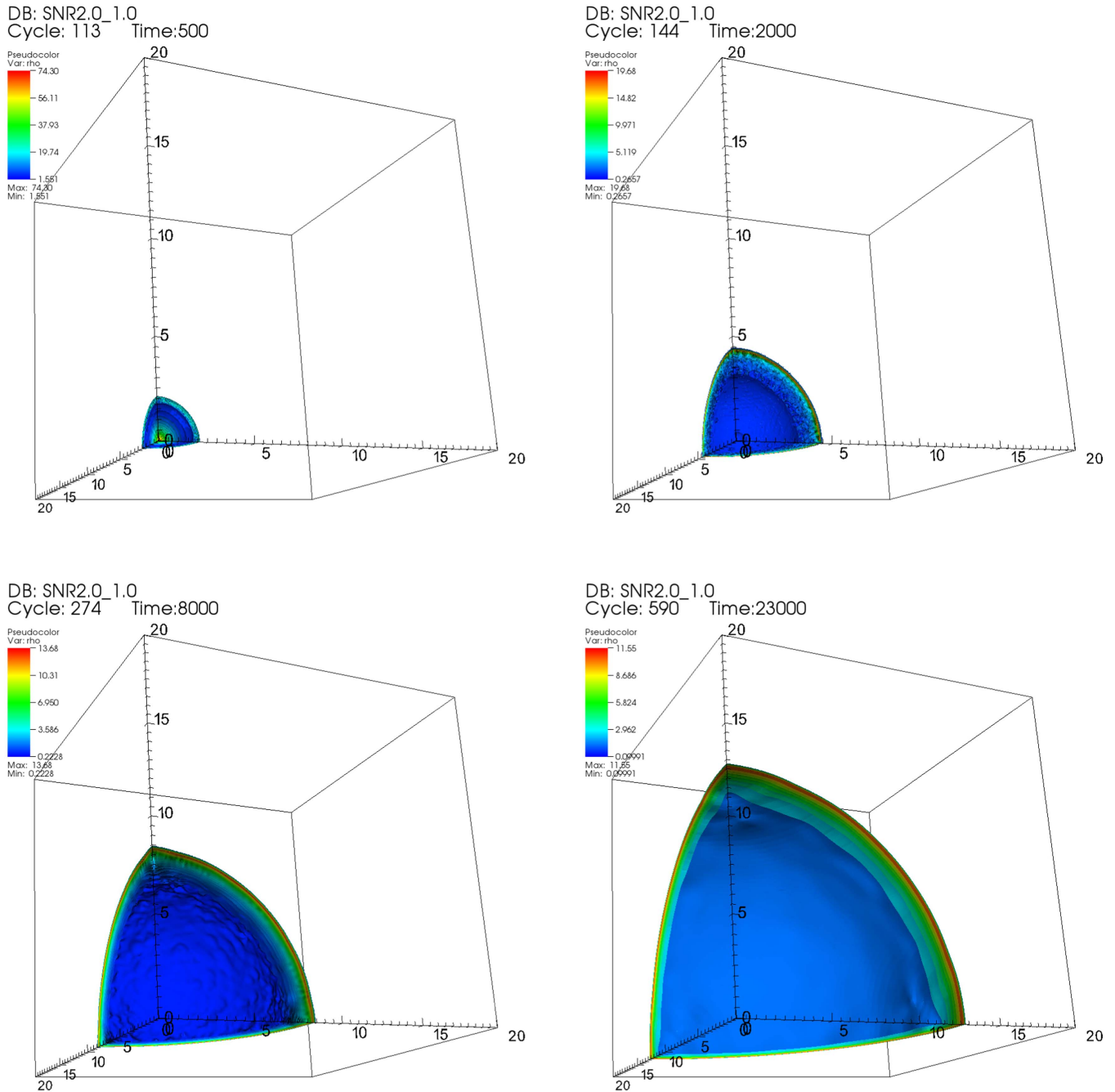
Figure 2. Simulation domain (SN explosion occurred at the origin of the one octant in the 3D Cartesian coordinate system (x_0, y_0, z_0) = (0, 0, 0) ). The colored regions mark particle number density. Series of density isosurfaces (3D surfaces containing cells with the same density value) depict hydrodynamic evolution corresponding to model SNR2.0_1.0 (see Table 1) at times t = 500 yr (upper left), 2000 yr (upper right), 8000 yr (lower left), and 23,000 yr (lower right). Contours correspond to linearly scaled values between the lowest and highest values sampled in the intershock region. The box is 20 pc along each axis. Effective AMR resolution varies from 8192^3 initially to 512^3 at the end of the simulation (23,000 yr).
