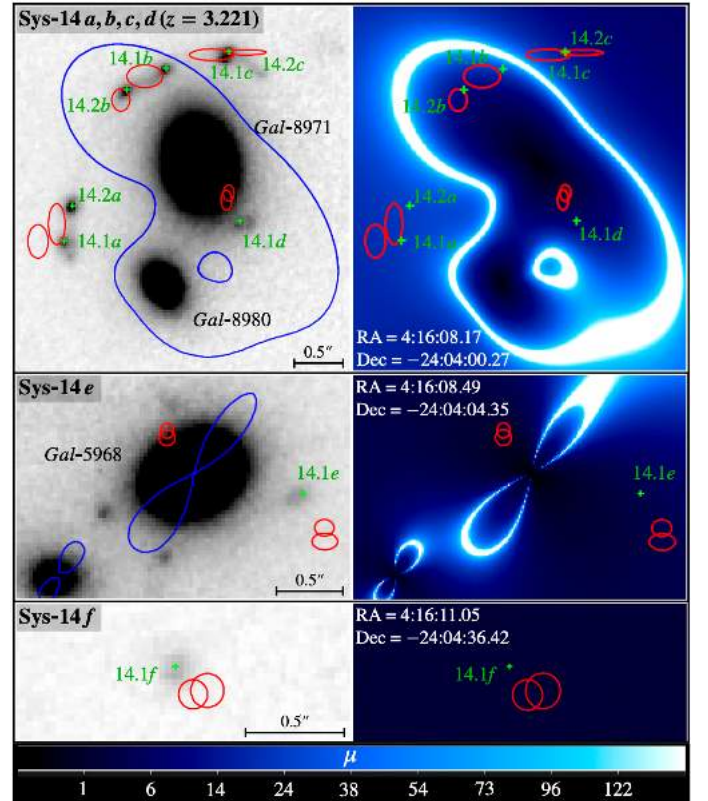
Fig. 13. Inspection of system 14 at z = 3.221 . A pair of nearly point-like clumps (14.1 and 14.2) is imaged six times by the cluster mass distribution, around two cluster galaxies ( Gal-8971 and Gal-8980 , with F160W magnitudes 19.6 and 21.5, respectively). Green crosses, red ellipses, and blue lines have the same meaning as Fig. 12. The three gray-scale cut-outs on the left are median stack images of F814W, F606W, and F435W HST filters. Right panels : absolute magnification ( \mu ) maps computed at z = 3.221 . The lens model predicts a fifth ( e ) and a sixth ( f ) image ( middle and bottom panels , see also Fig. 2).
