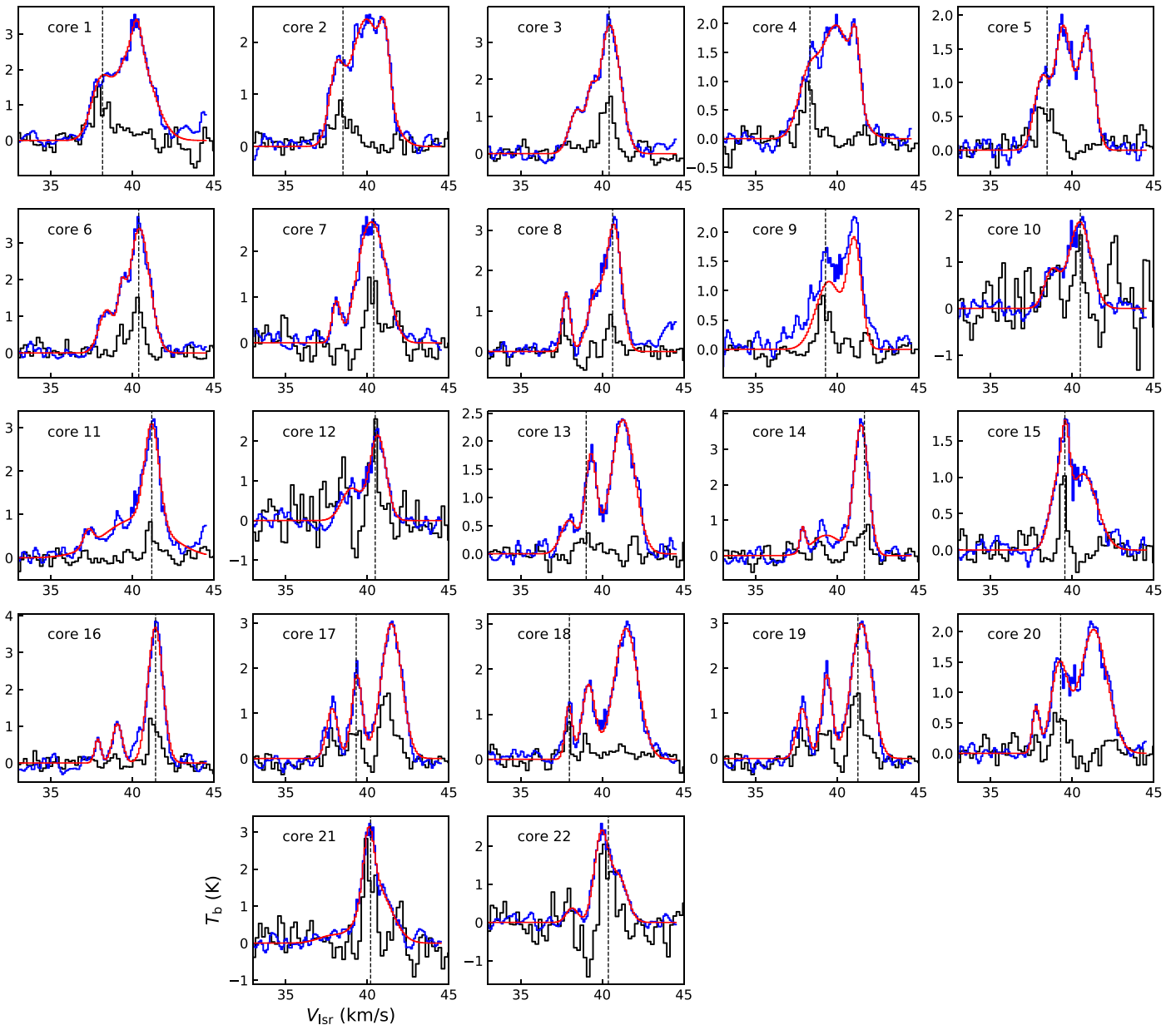
Figure 8. Comparison of the \text{N}_2\text{H}^+ ( 1-0 ), in blue, and the \text{o-H}_2\text{D}^+ ( 1_{1,0}-1_{1,1} ) spectra, in black, at the core positions. The spectra are taken at the position of the peak of \text{o-H}_2\text{D}^+ integrated intensity. The red curves show the best model obtained by fitting the \text{N}_2\text{H}^+ data with three Gaussian components. The centroid velocity of the \text{o-H}_2\text{D}^+ is shown with the vertical dashed line in each panel.
