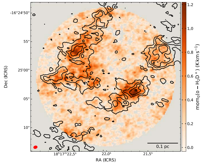
Figure 11. The color scale shows the integrated intensity of the \text{o-H}_2\text{D}^+(1_{1,0}\text{--}1_{1,1}) transition as in Figure 1. The black contours show the \text{N}_2\text{D}^+(3\text{--}2) integrated intensity (computed as for \text{o-H}_2\text{D}^+ ; see Section 2). The levels are: [7, 11, 15, 19]\sigma , where 1\sigma = 100 \text{ mK km s}^{-1} .
