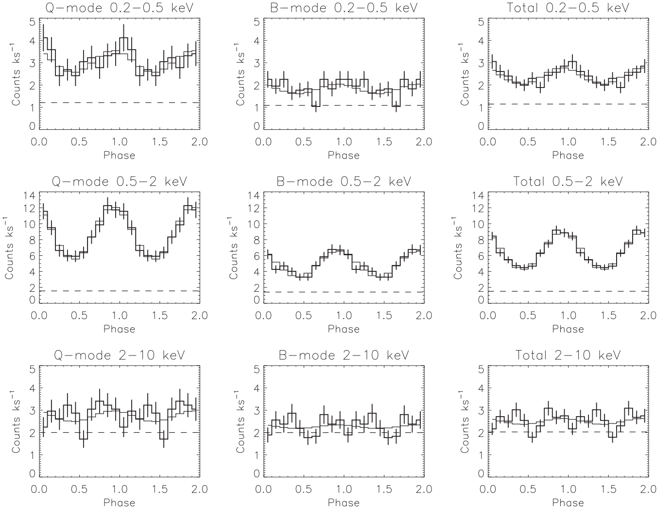
Figure 2. Folded pn+MOS light curves. The thin solid lines are the best-fit sinusoidal functions (with phase fixed to that determined from the Q-mode 0.5–2 keV pulse profile). The horizontal dashed lines indicate the background level.
