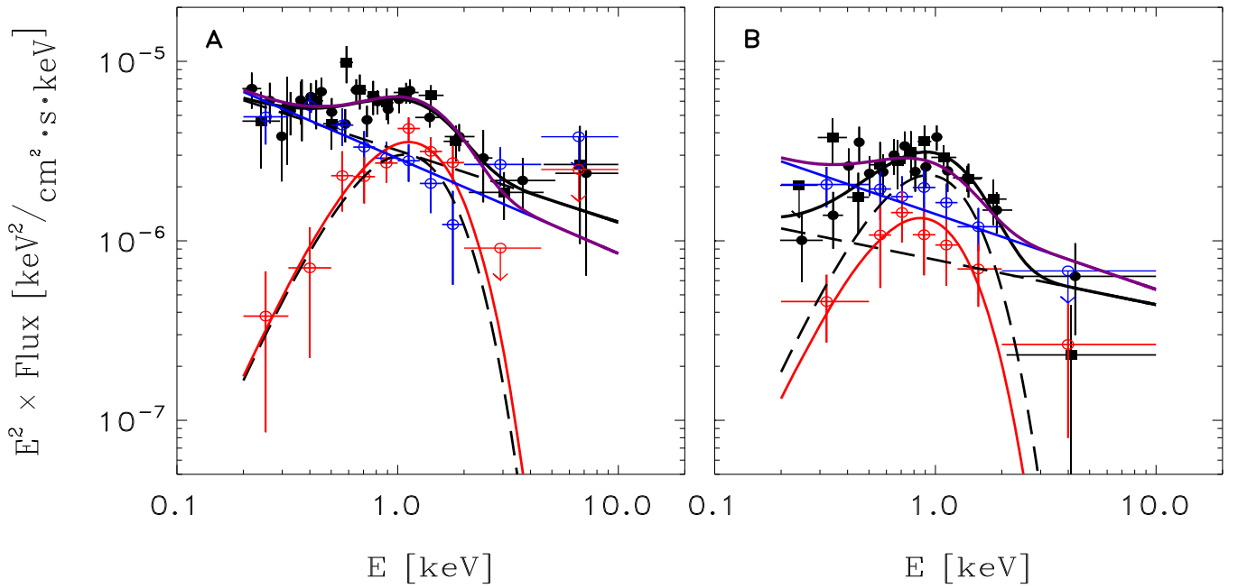
Figure 4. Results of the ML spectroscopy for the Q-mode (left panel) and B-mode (right panel). Black lines and points refer to the 2D-ML (circles pn, squares sum of the two MOS CCDs), solid lines are the best-fit blackbody plus power-law models, dashed lines the individual components). The results of the 3D-ML analysis are in blue for the unpulsed component (data points and best fit with a single power law) and in red for the pulsed component (data points and best fit with a single blackbody). The purple line is the sum of the blue and red lines.
