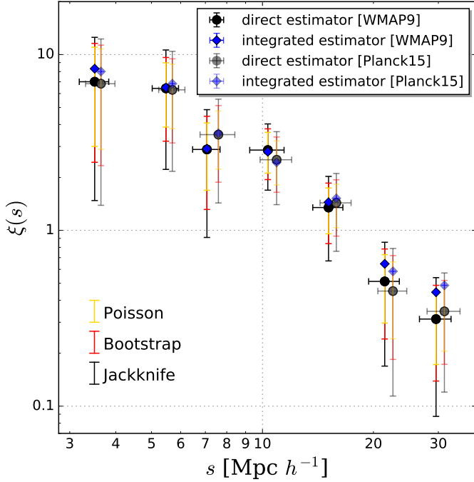
Fig. A.3. Comparison between the redshift-space 2PCF of XXL C1 clusters computed with the direct (dots) and integrated (diamonds) estimators, assuming either WMAP9 or Planck15 cosmologies (fuzzy coloured, slightly shifted for reasons of clarity). The error bars compare the Poisson, bootstrap, and jackknife estimated errors.
