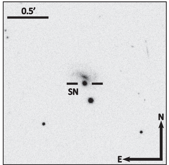
Figure 1. 2' \times 2' g' -band image from the 2.6 m Nordic Optical Telescope showing ASASSN-15nx and its host GALEXASC J044353.08-094205.8.
