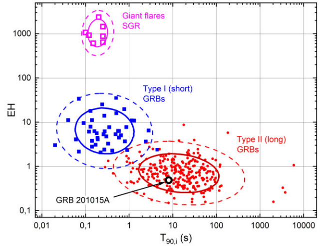
Figure 4. The T_{90,i} – EH diagram for type I (blue squares), type II (red circles) GRBs, and SGR giant flares (magenta unfilled squares) with corresponding cluster analysis results (68 per cent and 95 per cent confidence regions are shown by bold solid and thin dashed curves, respectively). GRB 201015A (black unfilled circle) is within the 68 per cent confidence region of type II GRBs.
