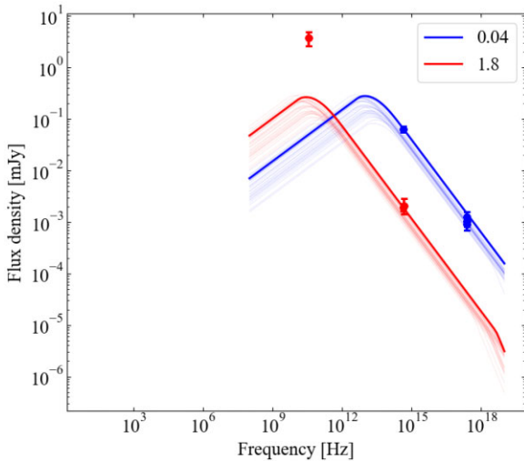
Figure 7. Spectral energy distribution of the GRB 201015A at epochs 0.04 and 1.8 d after detection. The results of the modelling are indicated by lines (see Section 3.2.3).
