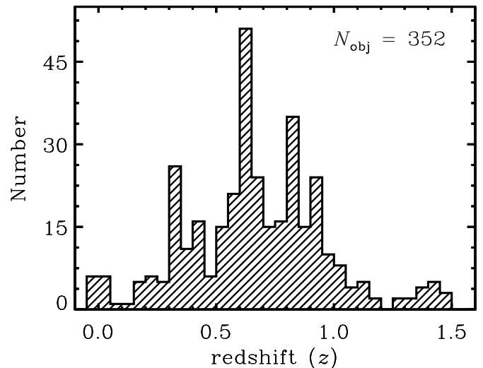
Figure 11. Distribution of the 352 unique, secure ( Q = -1, 3, 4 ) redshifts included in the Magellan/IMACS redshift catalog.
