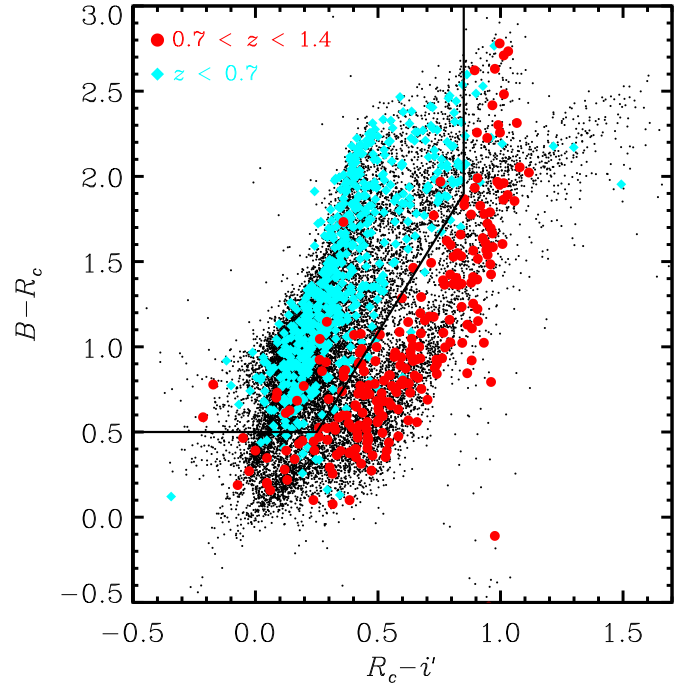
Figure 10. B - R_c vs. R_c - I color-color distribution for all sources with R_c < 23.5 in the Subaru imaging catalogs of Furusawa et al. (2008). The cyan and red points correspond to those objects with spectroscopic redshifts in the ranges z < 0.7 and 0.7 < z < 1.4 , respectively. The solid black lines show the color cuts employed to prioritize target selection (see Equation (A3)).
