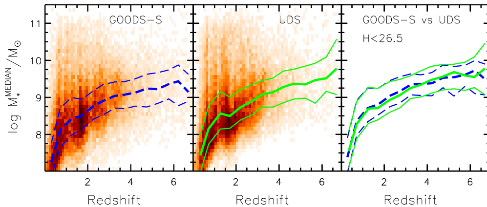
Figure 7. Reference median stellar mass (see Section 5.1) as a function of redshift in GOOD-S (left panel) and UDS (central panel). Colors and line styles are as in Figure 6. Thick lines show the median mass in bins of redshift ( \Delta z = 0.5 ), while thin lines show the semi interquartile range in the same bins. The right panel shows medians and semi interquartile ranges for the two samples cut at H_{160} < 26.5 .
