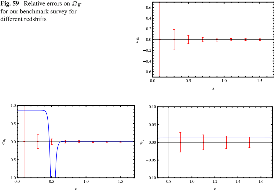
Fig. 60 Left: same as Fig. 59 but now with superimposed the prediction for the Lemaître–Tolman–Bondi model considered by García-Bellido and Haugbølle (2008a). Right: zoom in the high-redshift range
