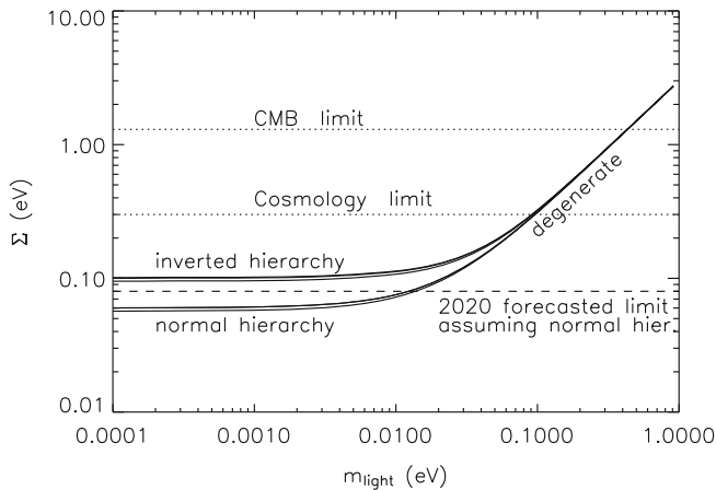
Fig. 41 Constraints from neutrino oscillations and from cosmology in the m – \Sigma plane. Image reproduced by permission from Jiménez et al. (2010); copyright by IOP and SISSA
