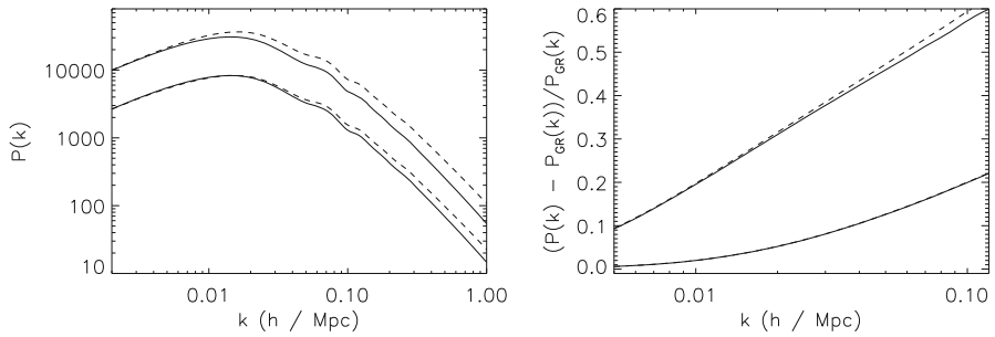
Fig. 32 Left panel: Linear matter power spectra for \Lambda CDM (solid line; M_0^{-1} = 0 , \nu = 1.5 ) and scalaron (dashed line; M_0^{-1} = 375 [10^{28} \text{ h}^{-1} \text{ eV}^{-1}] , \nu = 1.5 ) cosmologies. The modification to gravity causes a sizeable scale dependent effect in the growth of perturbations. The redshift dependence of the scalaron can be seen by comparing the top and bottom pairs of power spectra evaluated at redshifts z = 0.0 and z = 1.5 , respectively. Right panel: The environmental dependent chameleon mechanism can be seen in the mildly nonlinear regime. We exhibit the fractional difference (P(k) - P_{\text{GR}}(k))/P_{\text{GR}}(k) between the f(R) and GR power spectra for the model (1.8.37) with parameters M_0^{-1} = 375 [10^{28} \text{ h}^{-1} \text{ eV}^{-1}] and \nu = 1.5 . The dashed lines represent linear power spectra ( P(k) and P_{\text{GR}}(k) calculated with no higher order effects) and the solid lines are the power spectra calculated to second order. We see that the nonlinearities decrease the modified gravity signal. This is a result of the chameleon mechanism. The top set of lines correspond to z = 0 and the bottom to z = 0.9 ; demonstrating that the modified gravity signal dramatically decreases for larger z . This is due to the scalaron mass being much larger at higher redshifts. Furthermore, nonlinear effects are less significant for increasing z
