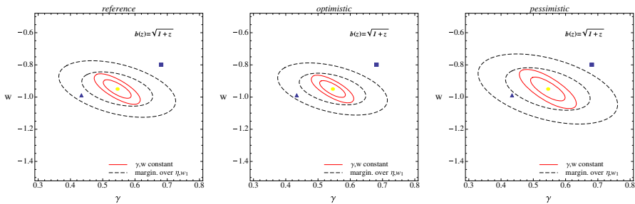
Fig. 22 \eta -parameterization. 1 and 2\sigma marginalized probability regions obtained assuming constant \gamma and w (red solid curves) or assuming the parameterizations (I.8.6) and (I.8.2) and marginalizing over \eta and w_1 (black dashed curves); marginalized error values are in columns \sigma_{\gamma_{\text{marg},2}} , \sigma_{w_{\text{marg},2}} of Table 9. Yellow dots represent the fiducial model, the triangles stand for a f(R) model and the squares mark the flat DGP
