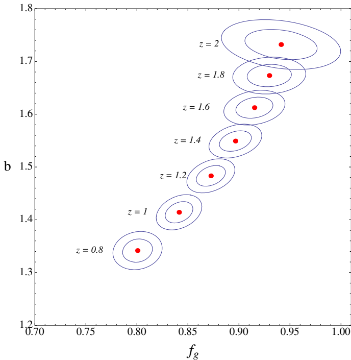
Fig. 17 Contour plots at 68 and 98% of probability for the pairs s(z_i) - b(z_i) in 7 redshift bins (with b = \sqrt{1+z} ). The ellipses are centered on the fiducial values of the growth rate and bias parameters, computed in the central values of the bins, z_i
