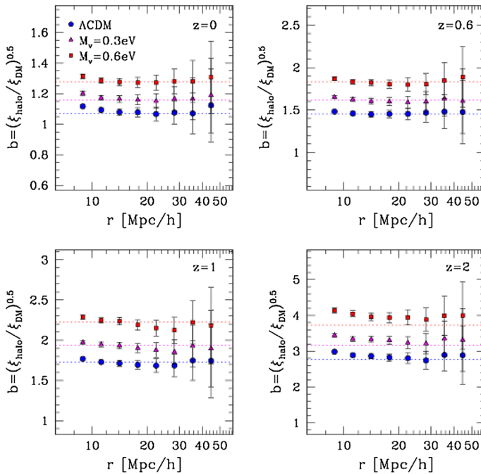
Fig. 45 Bias of the DM haloes in the \Lambda\text{CDM} N -body simulation (blue circles) and in the two simulations with \Sigma = 0.3 \text{ eV} (magenta triangles) and \Sigma = 0.6 \text{ eV} (red squares). Dotted lines are the theoretical predictions of Sheth et al. (2001)
