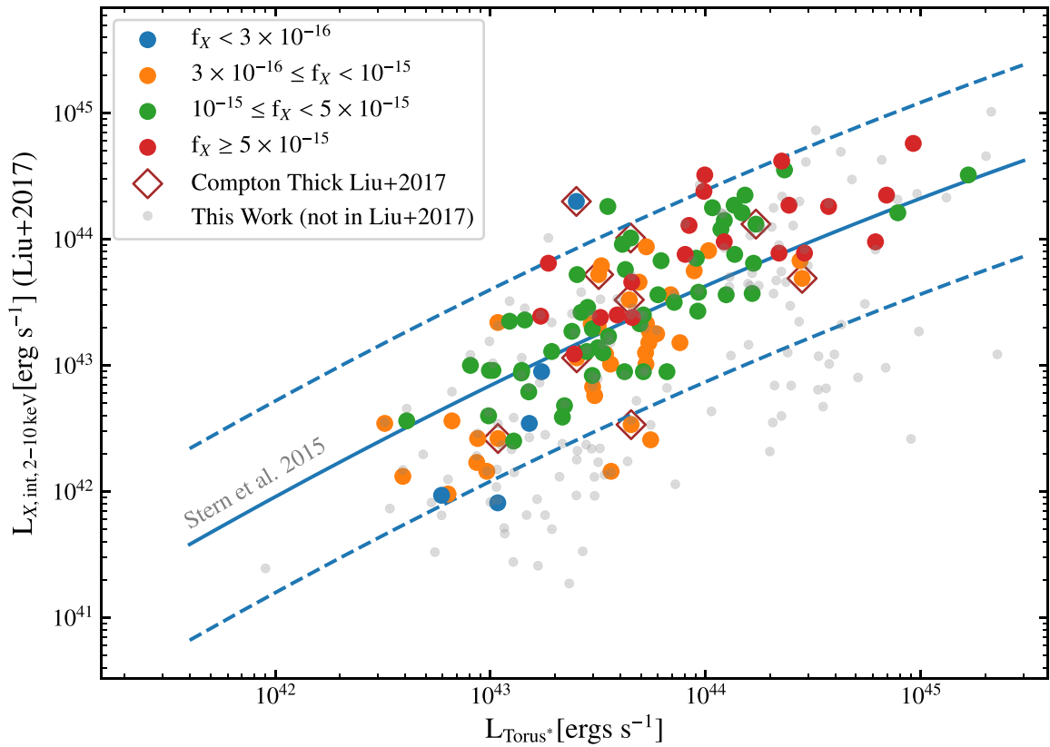
Figure 9. Shown is L_{X,int,2-10\text{ keV}} vs. L_{\text{Torus}^*} , where the absorption-corrected luminosities are provided from Liu et al. (2017). The points are color-coded by the X-ray flux provided in L17, and the fluxes have units of \text{erg s}^{-1} \text{cm}^{-2} . The blue solid line is the luminosity-dependent relationship from S15. Points surrounded by a red diamond are classified as Compton-thick in Liu et al. (2017). The gray points are the L_{X,int,2-10\text{ keV}} values from Figure 4 that did not have enough X-ray counts to be analyzed in Liu et al. (2017).
