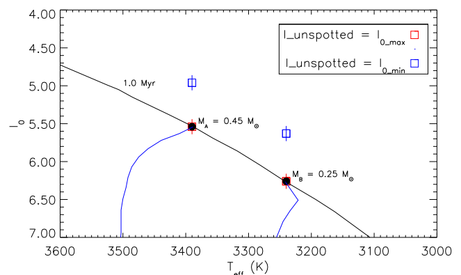
Figure 6. I_0 versus T_{\text{eff}} diagram of V1481 Ori. Black and blue solid lines represent theoretical isochrones and mass evolutionary tracks, respectively, from Baraffe et al. (1998). Black bullets represent the magnitudes expected from a model at 1 Myr. Red and blue open squares represent the observed magnitudes in the hypothesis that the unspotted magnitude corresponds to the faintest and brightest observed values, respectively.
