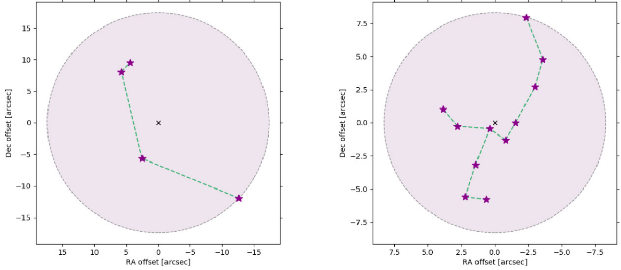
Figure 7. Example MST for fields SDC28.277–0.352.1 (left) and RMS-G050.2213–00.6063 (right), the same fields as shown in the maps in Fig. 3. Purple star icons denote source location, the green dashed lines are the edges of the MST. The purple shaded region is a circle of radius equal to the protocluster radius as defined in Section 3.2 centred at the average position of all sources in the field.
