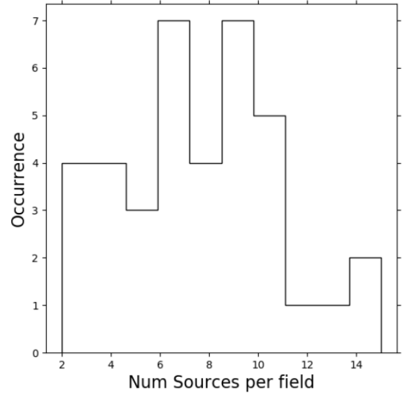
Figure 4. Distribution of fragment counts across the 38 TEMPO fields.
