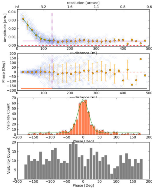
Figure C2. Simulated Gaussian source model visibility properties. The model has a SNR of 50 and major/minor axes of 2 arcsec. From top to bottom the panels give: (Top panel) and (second panel) as per Fig. C1. In the top panel the green line marks a Gaussian fit to the binned amplitude data. This is from the fit to measure the AG\_FWHM parameter. The vertical dashed line gives the 3\sigma limit of the Gaussian fit. In the second panel the vertical dashed line gives the same 3\sigma limit as in the top panel. The coral and grey lines are used to denote colours used in plotting phase histograms in the third and bottom panels. (Third panel) A histogram of the unaveraged phase values in the \leq 3\sigma uv -distance range (phase values with a uv -distance below the vertical dashed line in second panel). The green line describes a Gaussian fit to the data used to extract the ph1\_x0 and ph1\_FWHM parameters referred to in the text. (Bottom panel) A histogram of the unaveraged phase values at uv -distances > 3\sigma , the parameters for ph2\_x0 and ph2\_FWHM , are fit from data in this plot. In this specific case the fit is unsuccessful so now line is shown.
