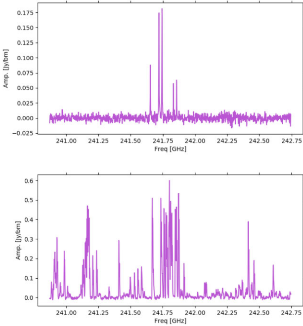
Figure 2. Examples of whole SPW (1.875 GHz bandwidth) spectra from the ALMA data. These examples present SPW 1 from a line ‘quiet’ field (top: SDC20.775–0.076.1, L_* = 6.5 \times 10^3 L_\odot ) and line dominated source (bottom: SDC35.063–0.726.1, L_* = 5.2 \times 10^3 L_\odot ). The spectra are taken at the position of the strongest continuum detection in the respective fields. The two brightest lines in the top panel are CH 3 OH (5 K –4 K ) transitions.
