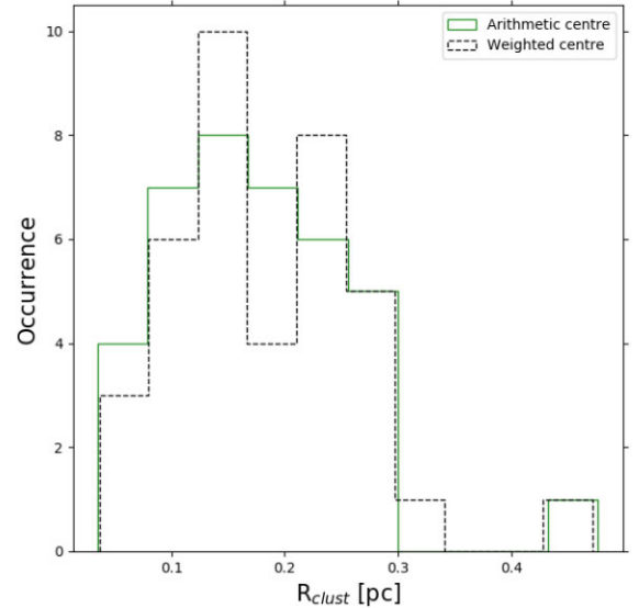
Figure 5. Distribution of measured cluster radii across the 38 fields in the TEMPO sample, as measured from the arithmetic mean position and weighted mean position.
