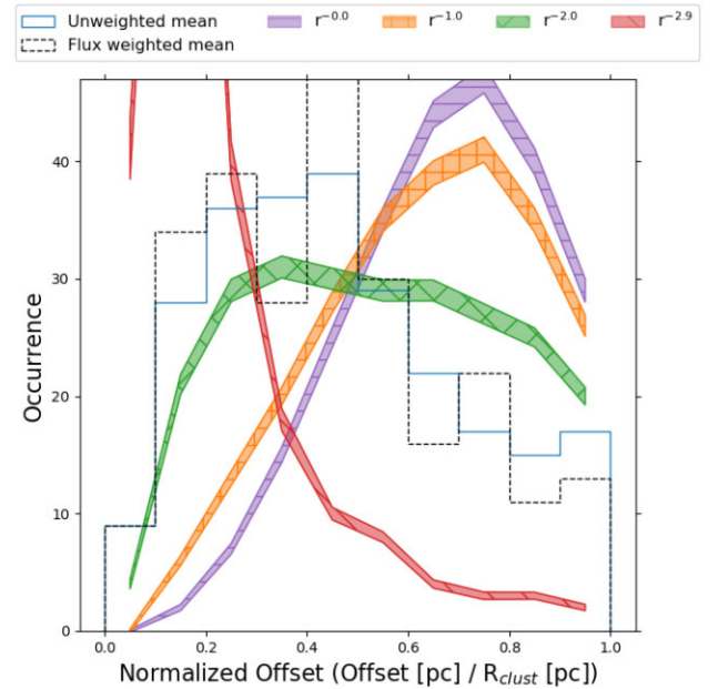
Figure 9. Combined distribution of source position as offset from the mean position of all fragments in their respective fields (blue histogram) and the normalized flux density-weighted mean position (black dashed histogram), normalized by the cluster radius R_{\text{clust}} or weighted cluster radius, for each field. The filled regions show the expected normalized radial profiles, r^{-\alpha} for values of \alpha = 0.0, 1.0, 2.0 , and 2.9 (purple with horizontal hatching, orange with ‘+’ hatching, green with ‘x’ hatching, and red with ‘\’ hatching, respectively). These profiles were drawn from 40 000 (10 000 per \alpha value) randomly generated three-dimension clusters with between 3 and 13 sources within them. See text for further details.
