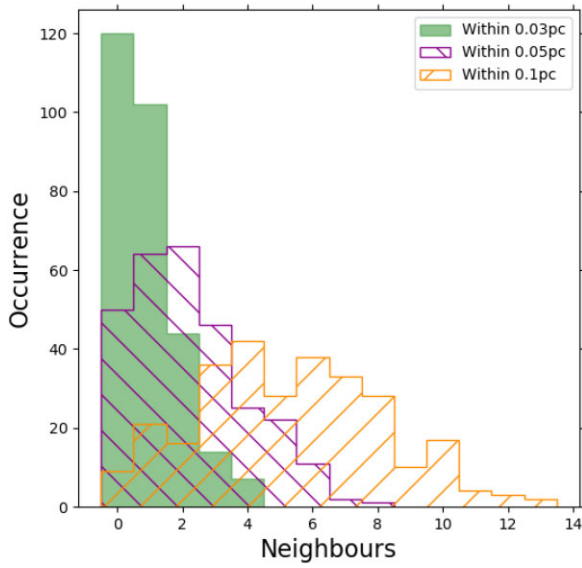
Figure 8. Number of nearest neighbours for each fragment in the sample at cutoffs of 0.03 pc (filled green histogram), 0.05 pc (purple ‘\’ hatched histogram) and 0.1 pc (yellow ‘/’ hatched histogram). Fragments in the Neighbours = 0 bin do not have a neighbour within that angular offset cut-off.
