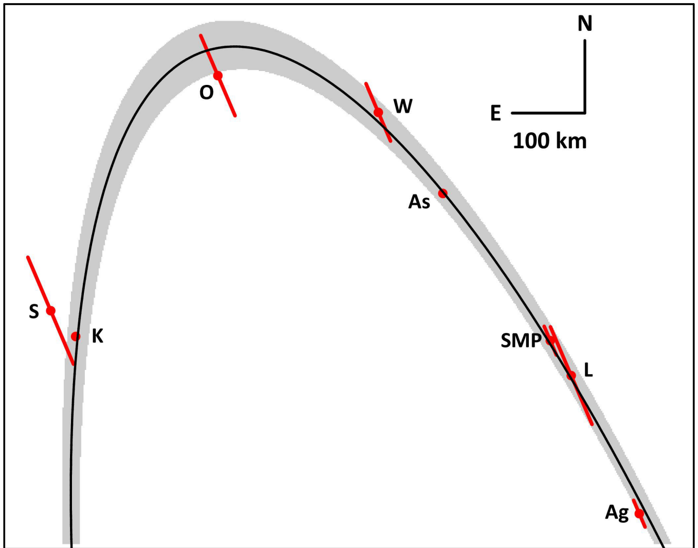
Extended Data Figure 4 | Upper part of the ring. An expanded view of Fig. 3 showing in more detail the events along the upper part of the ring. The best fitting mean ring radius a'_{\text{ring}} = 2,287^{+75}_{-45} km is drawn as a solid curve. The grey area shows the full extension of a semi-transparent
