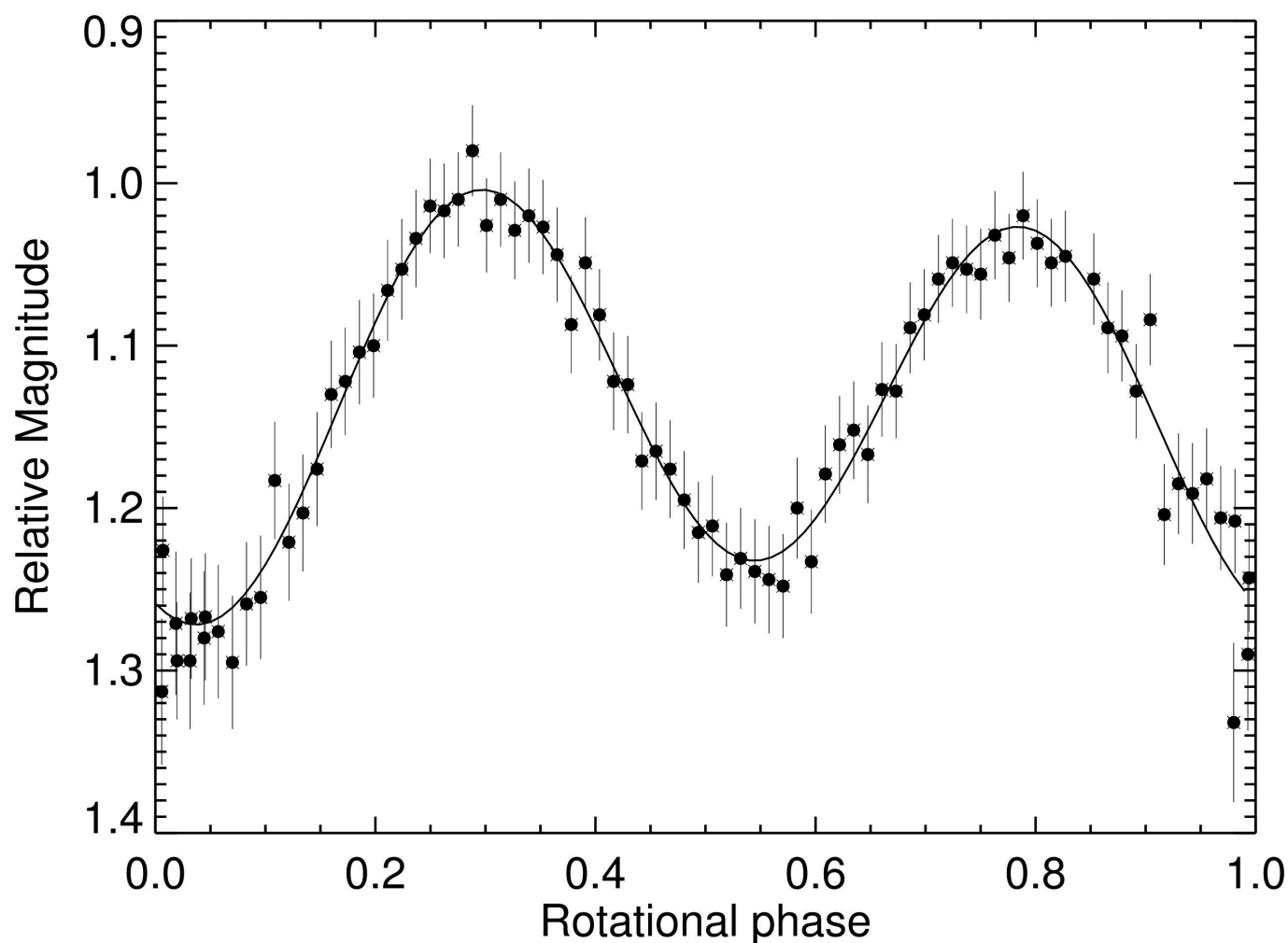
Extended Data Figure 6 | Rotational light curve of Haumea. The relative magnitude versus rotational phase obtained two days after the occultation with the Valle D'Aosta 0.81-m telescope with no filters is shown. The rotational zero phase was established at the time of the occultation and the rotation period used was 3.915341 h. Superimposed is a fit to the observational data. As can be seen, the absolute maximum in magnitude
