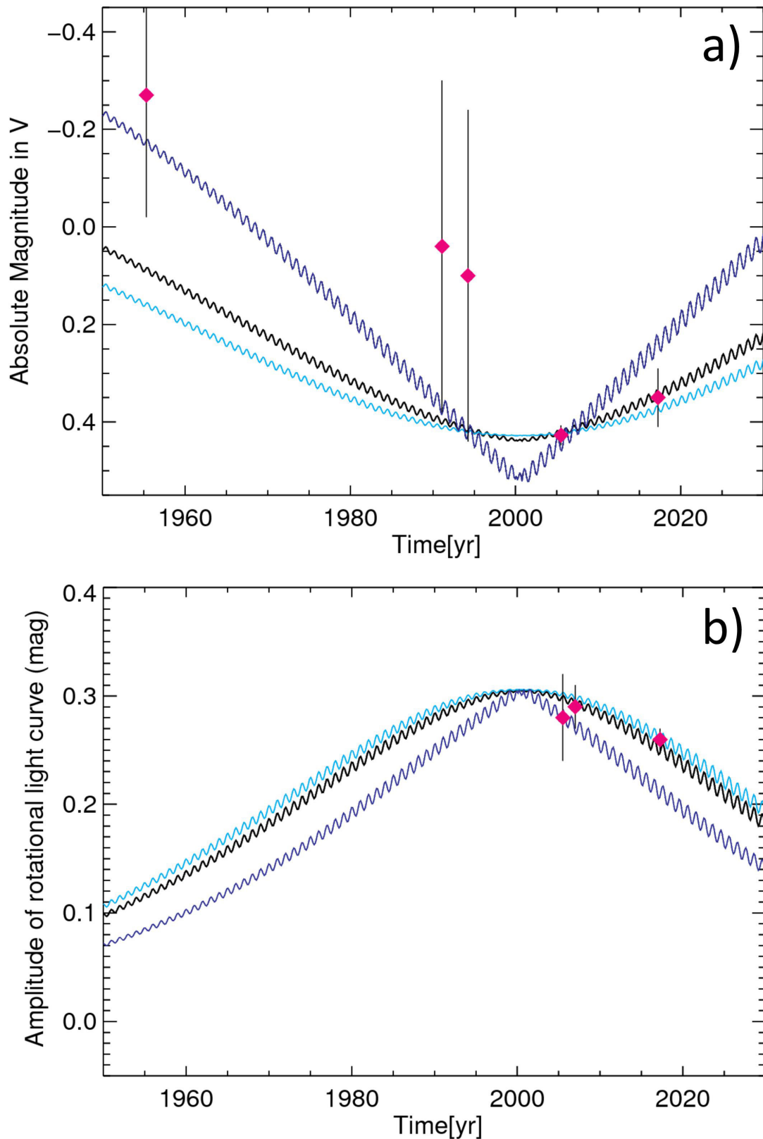
Extended Data Figure 5 | Photometric models. a , Absolute V-band magnitude of the Haumea system as a function of time. Diamonds represent observations and lines are models. The cyan curve represents a model without a ring, the black curve is a model with a 70-km-wide ring and with a reflectivity of I/F = 0.09 , similar to that of Chariklo's main ring. The ring in this model contributes approximately 2.5% of the total flux of Haumea plus Hi'iaka in 2017. The dark blue curve corresponds to a model with a wider (140 km) and brighter ( I/F = 0.36 ) ring, which contributes 20% of the total brightness in 2017. This model can be discarded because
