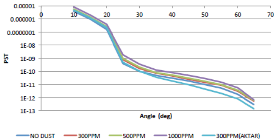
Figure 7: Stray light rejection calculations of the CHEOPS baffling system for different cleanliness levels. In addition, the stray light suppression capability is shown if improved black coating (Aktar) would be used.
