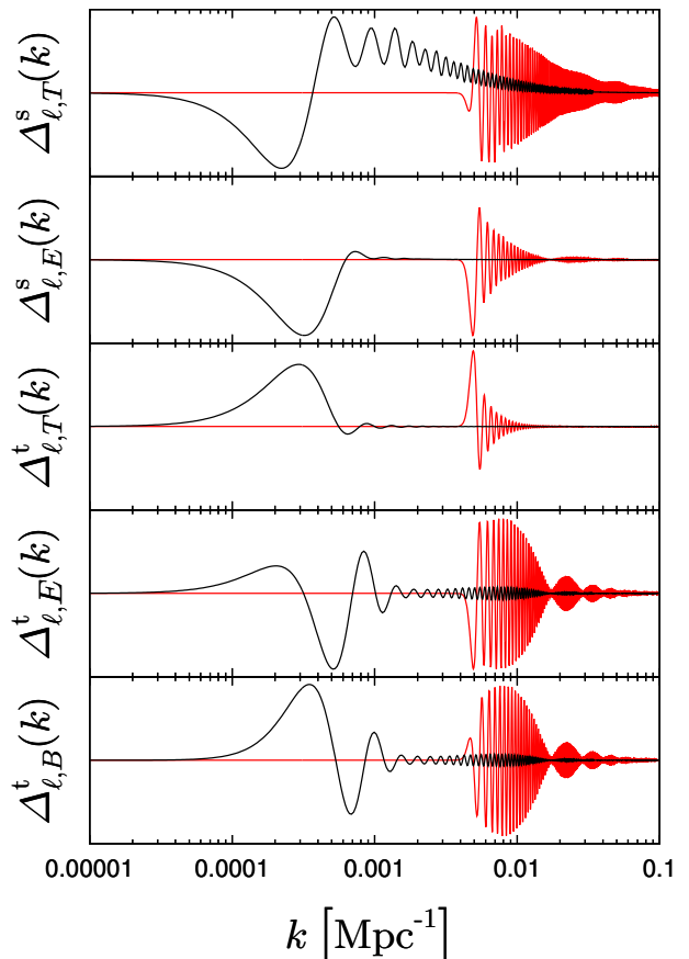
Fig. 1. Comparison of transfer functions for the scalar and tensor modes. The CMB transfer functions \Delta_{\ell, \mathcal{A}}^s(k) and \Delta_{\ell, \mathcal{A}}^t(k) , where \mathcal{A} = T, E, B , define the linear transformations mapping the primordial scalar and tensor cosmological perturbations to the CMB anisotropies as seen by us on the sky today. These functions are plotted for two representative values of the multipole number: \ell = 2 (in black) and \ell = 65 (in red).
