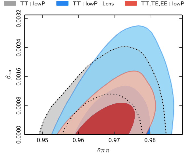
Fig. 52. Fully correlated ADI+CDI with n_{II} = n_{\mathcal{R}\mathcal{R}} (“curvaton I”). Since the spectral indices are equal, the primordial isocurvature fraction \beta_{\text{iso}} is scale independent.
