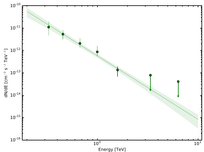
Figure 2. H.E.S.S. spectrum of PKS 0625–354 above 200 GeV. The panel presents best power-law fit to the data as a function of the true energy. Upper limits are given at 99 per cent confidential level with Feldman & Cousins (1998) confidence intervals. The green bow tie area gives the uncertainty of the fit at the 1\sigma confidence level.
