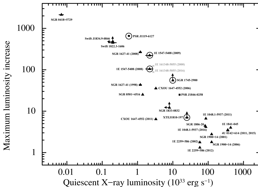
Figure 3. Maximum X-ray luminosity increase versus quiescent X-ray luminosity.
