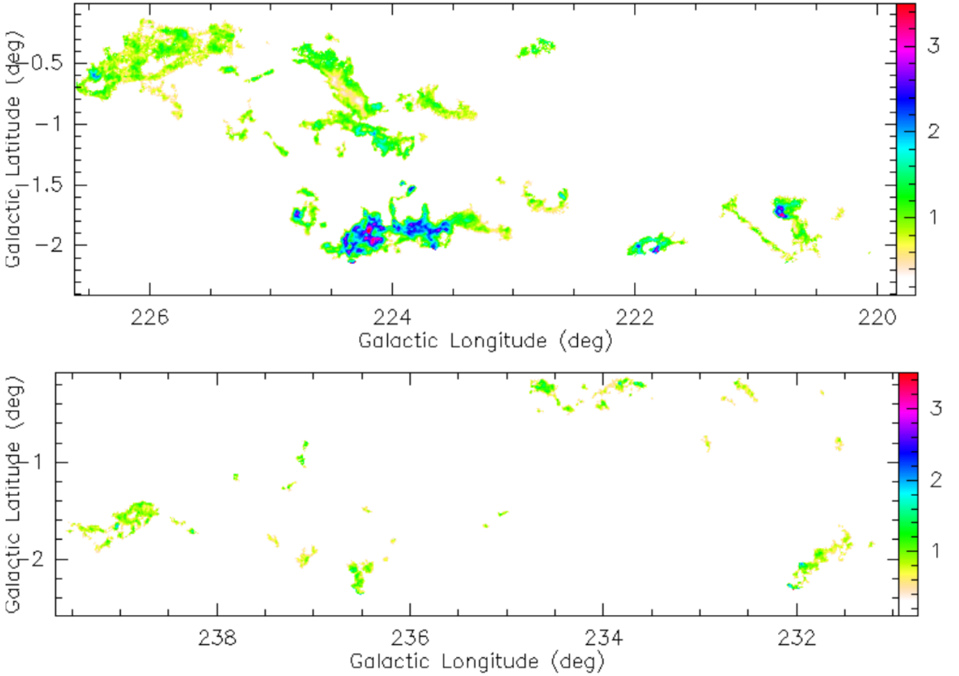
Fig. 3. N(\text{H}_2)_{N(^{13}\text{CO})}/N(\text{H}_2)_{\text{dust}} ratio (right colour bar) in the l = 220^\circ - 226^\circ 6' field (top) and that in the l = 231^\circ - 239^\circ 7' field (bottom).
