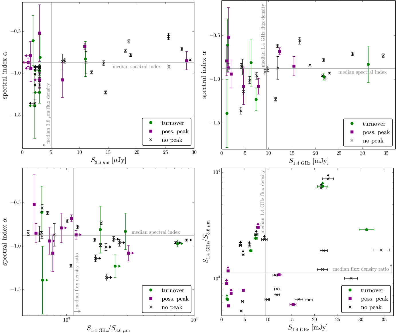
Fig. 4. Radio spectral index \alpha as a function of the 3.6 \mu\text{m} flux density ( top left ), \alpha as a function of the radio flux density S_{1.4 \text{ GHz}} ( top right ), \alpha as a function of the radio-to-IR flux density ratio S_{1.4 \text{ GHz}}/S_{3.6 \mu\text{m}} ( bottom left ), and S_{1.4 \text{ GHz}}/S_{3.6 \mu\text{m}} as a function of S_{1.4 \text{ GHz}} ( bottom right ) for our sample of 34 IFRS. The symbols distinguish subsamples of different turnover properties. Green dots represent sources with a detected turnover. Sources with a possible peak are shown by purple squares, and sources without a peak by black crosses. The classification is described in Sect. 3 and summarised for individual IFRS in Table 3. Upper and lower limits are represented by arrows. The grey horizontal and vertical lines indicate the medians or limits of the median.
