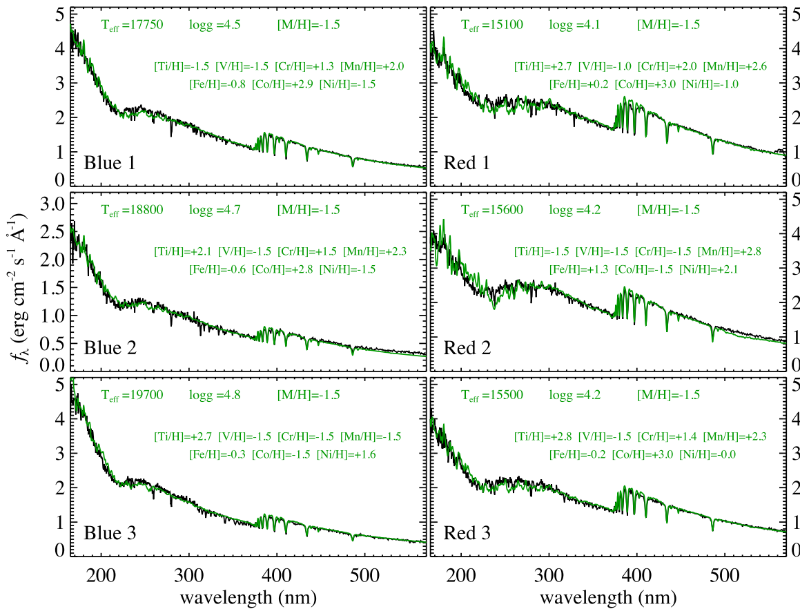
Figure 7. Spectra of our six stars (black curves) compared to the best-fit synthetic spectra (green curves) from ATLAS12 and SYNTH. In these models, most elements are held at the mean cluster abundance ( [M/H] = -1.5 ; Harris 1996), but seven elements (labels) near the Fe peak are allowed to vary up to an enhancement of 4.5 dex over the cluster value, because they can be significantly affected by radiative levitation (Michaud et al. 2011). The best-fit values in each fit (labels) are shown in Figure 8 to ease comparisons. The changes induced on each spectrum by the enhanced atmospheric metallicities are much larger in the red stars than in the blue stars (Figure 9).
