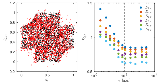
FIG. 5. Left: Phase-space portrait of the standard map as obtained from the raw time series (\theta_t, \theta_{t+1}) (black) and from reconstructions of empirical modes (\theta_t^*, \theta_{t+1}^*) up to k^* = 6 (red). Right: Behavior of the multiscale generalized fractal dimensions D_{q,\tau} vs. the timescale \tau for q \in [0, 5] . The gray dashed line marks the timescale \tau^* at which the multiscale generalized dimensions D_{q,\tau} converge to the fractal dimensions D_q .
