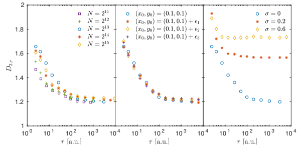
FIG. 2. Behavior of the multiscale generalized fractal dimension D_{2,\tau} for the Hènon map in dependence on the timescale \tau for different number of iterations N (left panel), different initial conditions (middle panel, N = 2^{13} , \epsilon_i < \epsilon = 0.01 for i = 1, 2, 3 ), and different noise levels \sigma (right panel, N = 2^{13} ).
