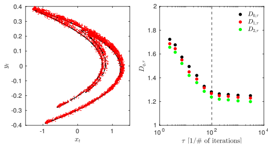
FIG. 1. Left: Phase-space portrait of the Hènon map based on the raw time series (black) and empirical mode reconstructions (red) using partial sums of Eq. (12) up to k^* = 7 . Right: Behavior of the multiscale generalized fractal dimensions D_{q,\tau} in dependence on the timescale \tau . The gray dashed line marks the timescale \tau^* at which the multiscale generalized dimensions D_{q,\tau} converge to the expected fractal dimensions D_q .
