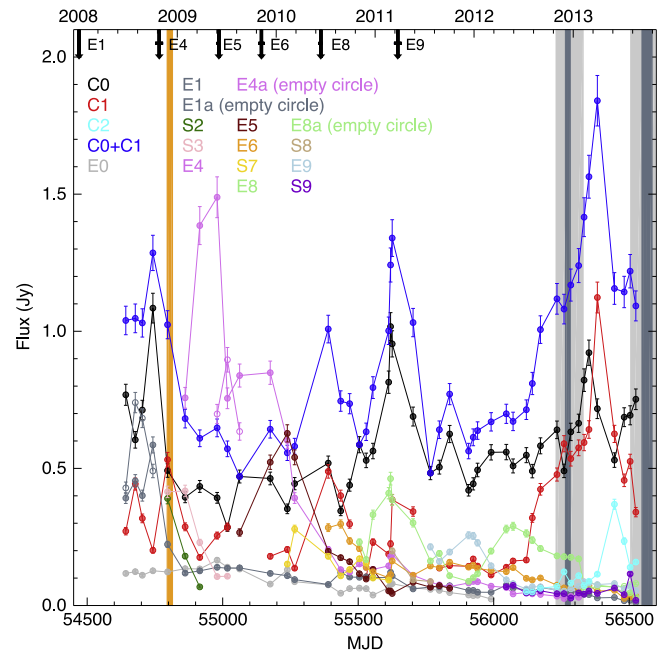
Figure 4. Light curves of the 15 GHz model-fit components, including the added total flux density of the core and component C1 (C0+C1). Arrows and vertical lines are as indicated in Figure 3.
