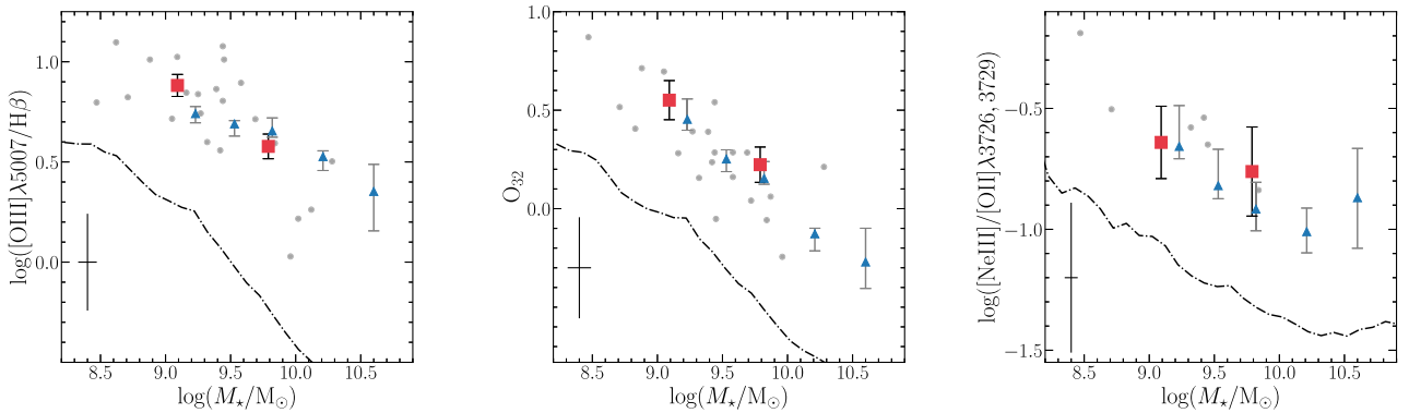
Figure 7. Dust-corrected emission lines ratios versus M_* for galaxies at z \approx 3.4 and z \approx 0 . Each panel shows one of the three emission-line ratios used to determine Z_g in this paper (see Section 3). From left to right, these line ratios are [\text{O III}]\lambda 5007/\text{H}\beta , \text{O}_{32} , and [\text{Ne III}]\lambda 3726, 3729 . The red squares show the low- M_* and high- M_* NIRVANDELS stacks (see also Fig. 5) and the grey circles show the individual NIRVANDELS galaxies with the necessary line detections. The median error bar on the individual detections is shown in the bottom left-hand corner. The blue triangular data points show stacked measurements from the z \approx 3.3 MOSDEF sample presented in Sanders et al. (2020a). The dot–dashed lines represent the running medians for z \approx 0 galaxies from the SDSS sample of Andrews & Martini (2013). These z \approx 0 line ratios have been corrected, where possible, for diffuse ionized gas (DIG) contamination that can bias line flux measurements in local galaxies [see the text and Sanders et al. (2020a) for further details].
