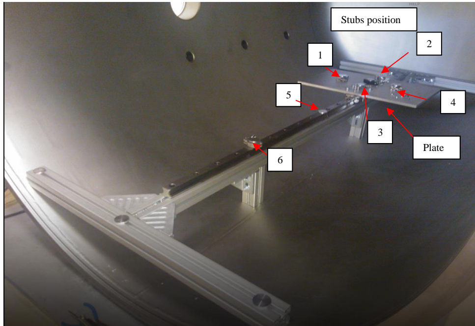
Figure 2 Aluminum Stub with Carbon Disc inside the simulation chamber in order to verify the particles distribution
