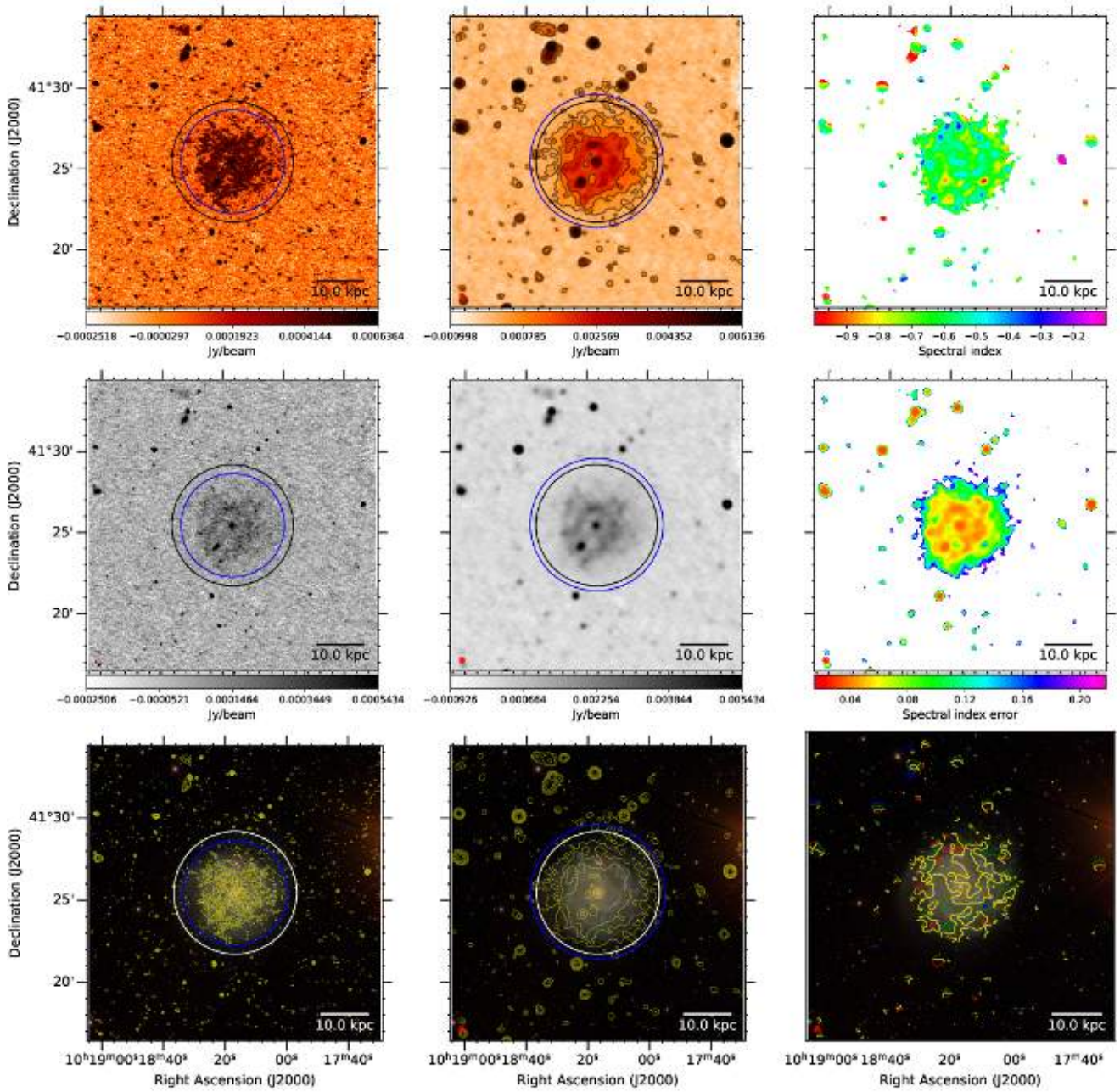
Fig. B.14. NGC 3184. The first row shows from left to right the 144-MHz maps at 6 and 20 arcsec resolution, respectively, and the radio spectral index map between 144 and 1365 MHz at 20 arcsec resolution. Contours start at 3\sigma with increments of a power of two. The black circle shows the optical D_{25} diameter and the blue ellipses show the 3\sigma contour extent used to integrate the flux density. The second row shows again the 6- and 20-arcsec images without contours and the radio spectral index error. The third row shows the 6- and 20-arcsec contours overlaid on an rgb SDSS image as well as contours of the radio spectral index. The filled circle shows the synthesised beam. A scale bar shows the projected size at the distance of the galaxy.
