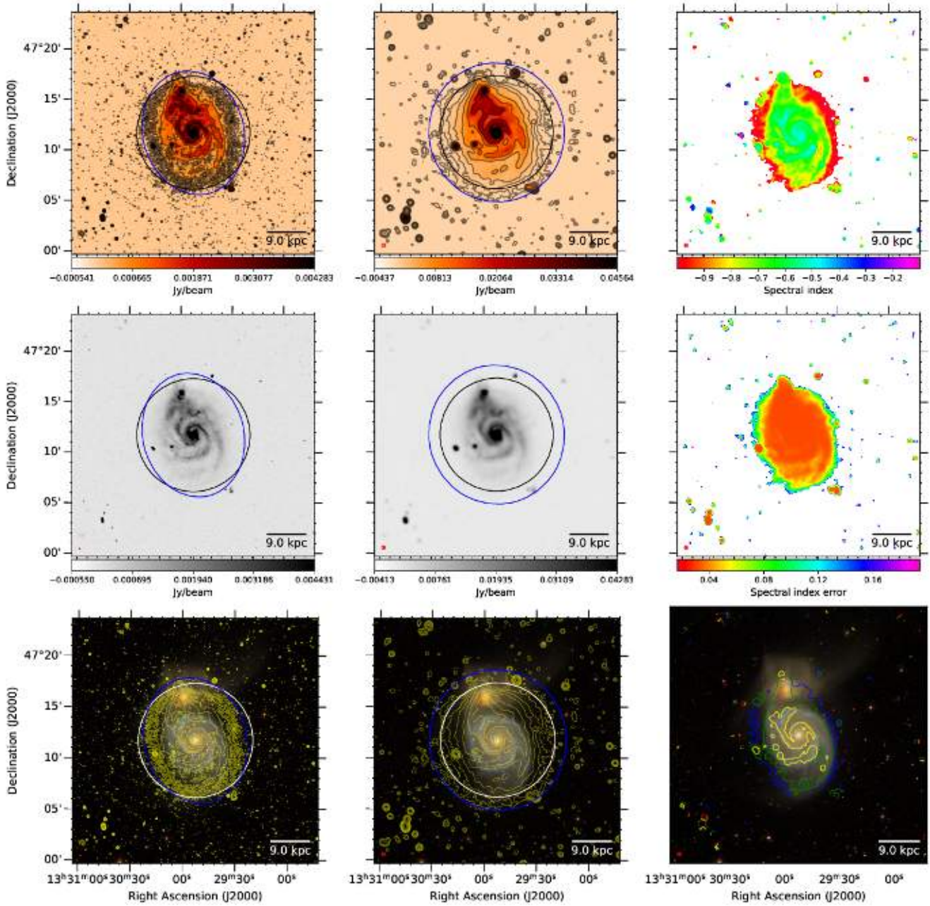
Fig. 2. NGC 5194 (M51). The first row shows from left to right the 144-MHz maps at 6 and 20 arcsec resolution, respectively, and the radio spectral index map between 144 and 1365 MHz at 20 arcsec resolution. Contours start at 3\sigma with increments of a power of two. The black circle shows the optical D_{25} diameter and the blue ellipses show the 3\sigma contour extent used to integrate the flux density. The second row shows again the 6 and 20 arcsec images without contours and the radio spectral index error. The third row shows the 6 and 20 arcsec contours overlaid on an rgb SDSS image as well as contours of the radio spectral index. Contours are at -1.0 (blue), -0.8 (green), -0.6 (yellow), and -0.4 (red). The filled circle shows the synthesised beam. The scale bar shows the projected size at the distance of the galaxy.
