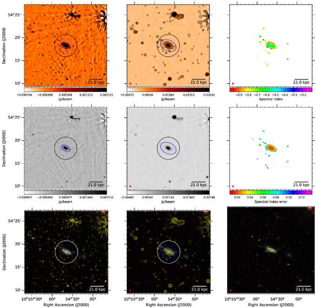
Fig. B.19. NGC 3448. The first row shows from left to right the 144-MHz maps at 6 and 20 arcsec resolution, respectively, and the radio spectral index map between 144 and 6000 MHz at 20 arcsec resolution. Contours start at 3\sigma with increments of a power of two. The black circle shows the optical D_{25} diameter and the blue ellipses show the 3\sigma contour extent used to integrate the flux density. The second row shows again the 6- and 20-arcsec images without contours and the radio spectral index error. The third row shows the 6- and 20-arcsec contours overlaid on an rgb SDSS image as well as contours of the radio spectral index. The filled circle shows the synthesised beam. A scale bar shows the projected size at the distance of the galaxy.
