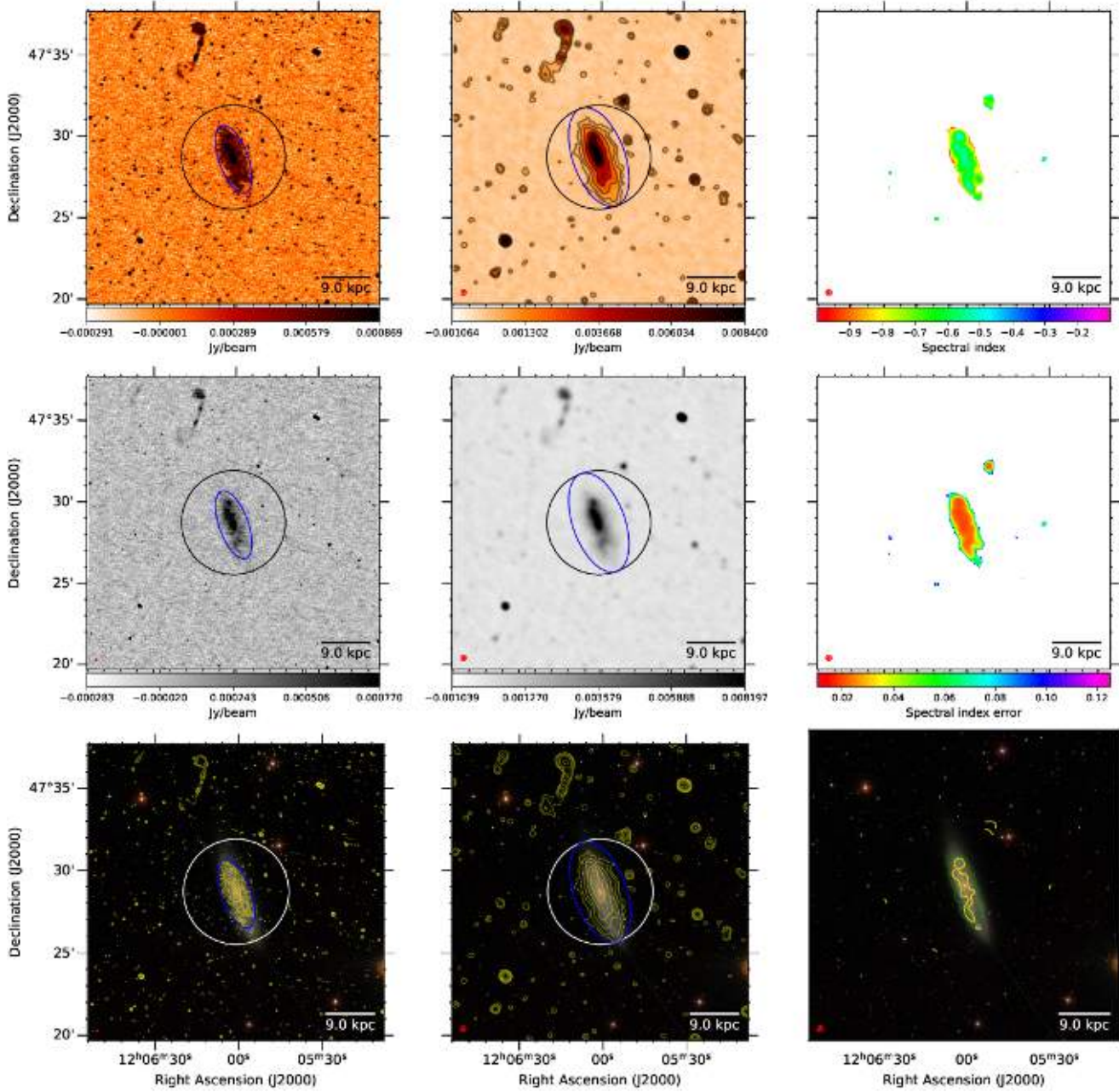
Fig. B.24. NGC 4096. The first row shows from left to right the 144-MHz maps at 6 and 20 arcsec resolution, respectively, and the radio spectral index map between 144 and 6000 MHz at 20 arcsec resolution. Contours start at 3\sigma with increments of a power of two. The black circle shows the optical D_{25} diameter and the blue ellipses show the 3\sigma contour extent used to integrate the flux density. The second row shows again the 6- and 20-arcsec images without contours and the radio spectral index. The filled circle shows the synthesised beam. A scale bar shows the projected size at the distance of the galaxy.
