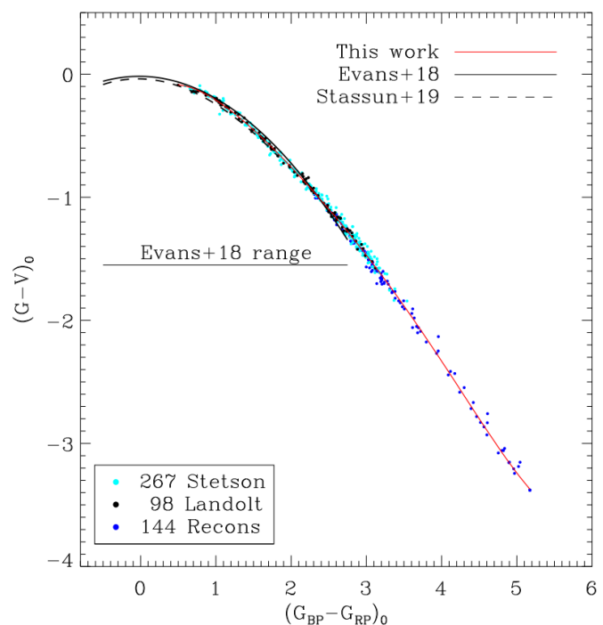
Fig. A.1. Relationship between the intrinsic (G-V)_0 and (G_{BP}-G_{RP})_0 colours calibrated in this work (solid red line). We also show the corresponding Evans et al. (2018) (solid black line) and Stassun et al. (2019) (dashed black line) relationships.
