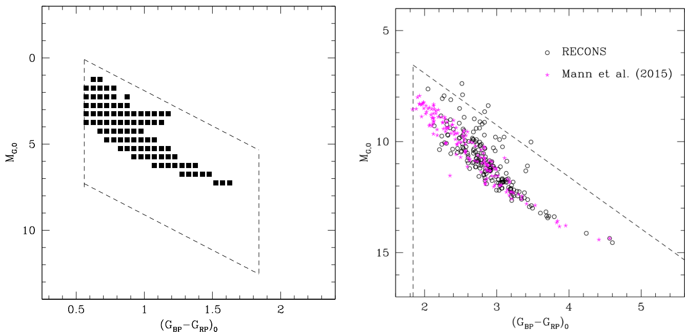
Fig. 4. In the left panel, black rectangles represent FGK dwarfs and subgiants from RAVE (see Sect. 3.2, Kunder et al. 2017). The right panel shows M-dwarfs (Henry et al. 2018, open circles) and Mann et al. (2015, magenta asterisks) catalogues. Dashed lines in both panels show the analytical selection defined in Sect. 3.3 for the FGK (left) and M stellar samples (right).
