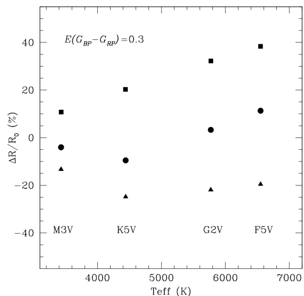
Fig. F.2. Percentage variation of the apparent radius R estimated neglecting the presence of both absorption and reddening (dots) for stars of different spectral types and for a reddening equal to E(G_{BP} - G_{RP})=0.3 . Squares and triangles represent the percentage radius variation resulting from neglecting the reddening or the absorption, respectively.
