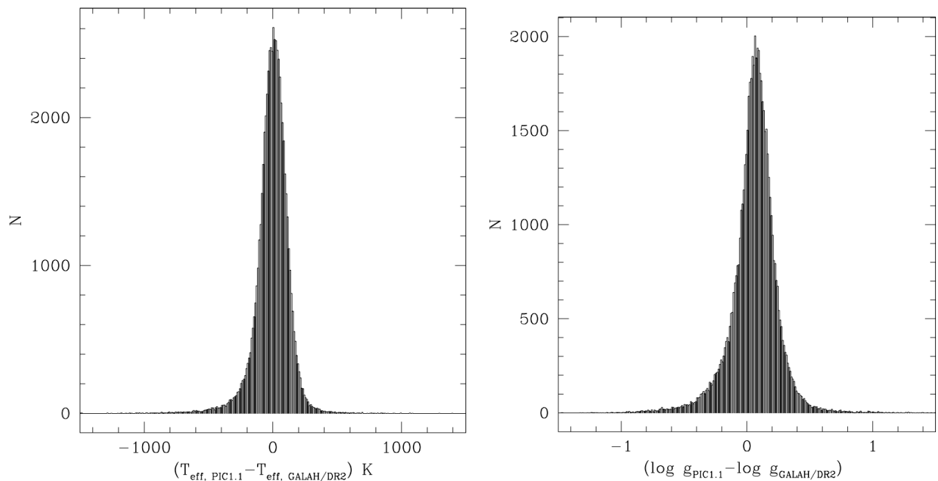
Fig. 17. Distributions of effective temperatures, and stellar gravity differences between asPIC1.1 and GALAH/DR2.
