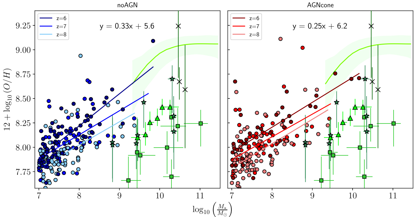
Figure 4. Stellar mass–metallicity relation for \text{noAGN} (left-hand panel; blue, light blue, and cyan points for z = 6, 7, 8 , respectively) and \text{AGNcone} (right-hand panel; red, light red, and pink points for z = 6, 7, 8 , respectively). A linear fit of the same colour is superimposed to each distribution. The best-fitting equations for z = 6 populations are y = 0.33x + 5.6 and y = 0.25x + 6.2 for \text{noAGN} and \text{AGNcone} , respectively. For comparison, we plot over each panel some of M_* - Z relations from the gas phase in star-forming galaxies: Mannucci et al. (2010) at z = 0 (light green line with a shaded region representing 90 per cent of the SDSS galaxies), Cullen et al. (2014) at z \gtrsim 2 (triangles), Maiolino et al. (2008) at z \sim 3.5 (squares), Faisst et al. (2016) at z \sim 3.5 (stars), and Harikane et al. (2020) at z \sim 6 (crosses).
