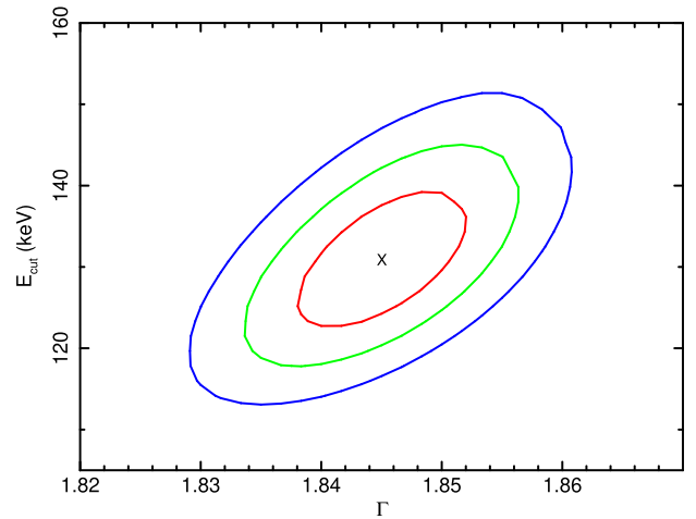
Figure 5. Contour plot E_{\text{cut}} - \Gamma for the broad-band model. The red, green, and blue lines represents the 68 per cent ( 1\sigma ), 95 per cent ( 2\sigma ), and 99.7 per cent ( 3\sigma ) confidence levels, while the best-fitting value is marked by an X.
