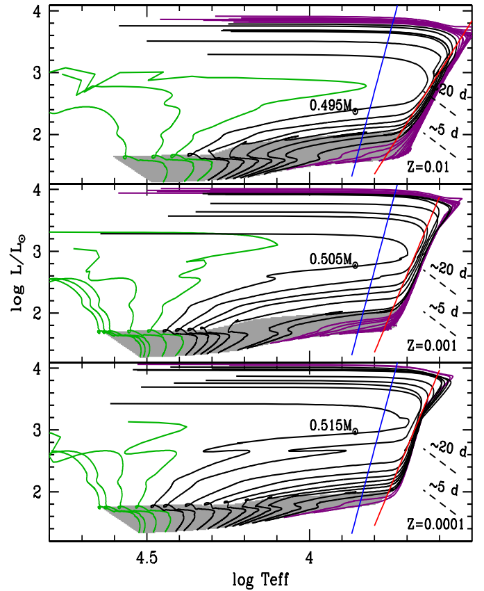
Fig. 5. Top: HRD of HB evolutionary models covering a broad range of stellar masses ( M/M_{\odot} = 0.48\text{--}0.90 ) and the same initial chemical composition ( Z = 0.01 , Y = 0.259 ). The grey area outlines the region between ZAHB (faint envelope) and central helium exhaustion (bright envelope). The green lines display HB models evolving as AGB-manqué, black lines the post early-AGB models, and purple lines the thermal pulsing AGB models (see text for details). The almost vertical blue and red solid lines indicate the hot and cool edges of the Cepheid instability strip. The minimum stellar mass (in solar units) crossing the instability strip is labelled in black. The black dashed lines show two iso-periodic lines for 5 and 20 days. Middle: same as the top panel, but for stellar masses ranging from M/M_{\odot} = 0.4912 to 0.80 and for a metal-intermediate chemical composition ( Z = 0.001 , Y = 0.246 ). Bottom: same as the top panel, but for stellar masses ranging from M/M_{\odot} = 0.5035 to 0.70 and for a metal-poor chemical composition ( Z = 0.0001 , Y = 0.245 ).
