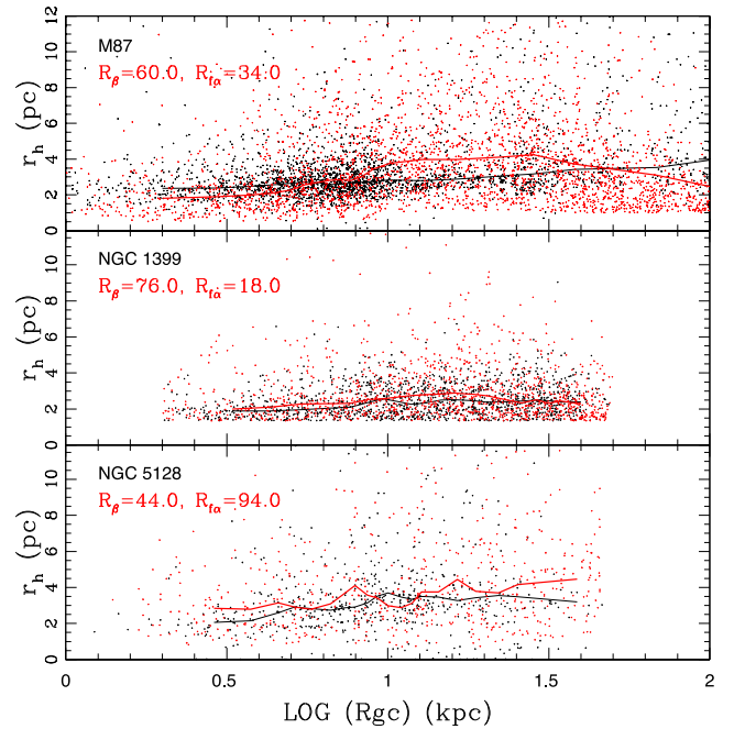
Figure 4. r_h versus \log R_{gc} for observed globular clusters (black) and model clusters (red) in M87 (top), NGC 1399 (middle), and NGC 5128 (bottom). Model clusters have anisotropy and tidal filling profiles as given by equations (4) and (5), with the best-fitting values of R_\beta and R_{f\alpha} indicated in each panel. The solid lines represent the median r_h calculated with radial bins containing 5 per cent of the observed cluster population.
