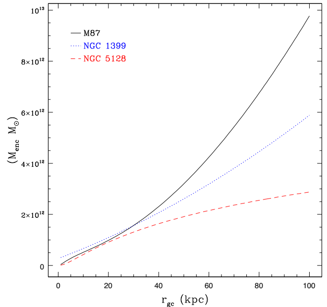
Figure 1. Total enclosed mass as a function of r_{\text{gc}} for M87 (black), NGC 1399 (blue), and NGC 5128 (red).
