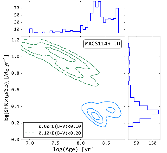
Figure 12. Distribution of galaxy age vs. star formation rate for MACS 1149-JD ( z_{\text{phot}} = 9.3 ) from our Monte Carlo simulations. We plot the estimated number density contours for Monte Carlo realizations with different ranges of E(B - V) values in the central panel to show the correlation between galaxy age, dust attenuation, and star formation rate. We also show the marginalized histograms of star formation rate on the right, and we show the marginalized histograms of galaxy age on the top. The star formation rate is the intrinsic value assuming a magnification factor of 5.5 for MACS 1149-JD.
