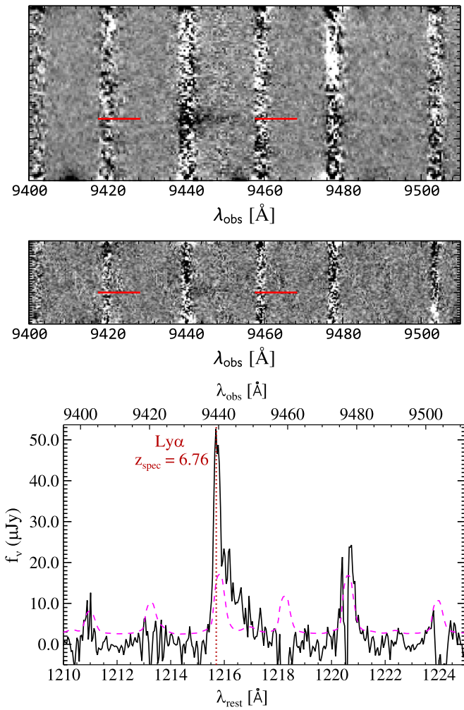
Figure 6. Reduced two-dimensional (top and middle panels) and one-dimensional (bottom panel) spectrum of RXJ 1347-1216. The top panel shows the data taken with the 8301 \text{ mm}^{-1} grating on 2013 April 3, and the middle panel shows the data taken with the 12001 \text{ mm}^{-1} grating on 2014 May 26. The one-dimensional spectrum was extracted from the 8301 \text{ mm}^{-1} spectrum. We also plot the rms spectra in dashed lines and mark the emission line redshift if the line is to be Ly \alpha . The flux density values given on the ordinate are calculated in the rest-frame assuming the line to be Ly \alpha .
