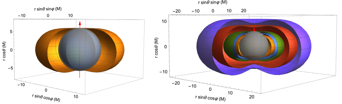
FIG. 6. Left panel: Critical hypersurfaces for the case of a rotating NS with Kerr parameter a = 0.41 (orange, f_\star = 600 Hz, \Omega_\star = 0.031 M^{-1} ) and for the nonrotating case (blue). For a nonrotating NS, the critical radius is constant and it takes unphysical value of r_{\text{crit}} \sim 5.56M . In the case of a rotating NS, the critical radius takes the value r_{\text{crit}}^{\text{eq}} \sim 12.05M in the equatorial plane, while it takes the value of r_{\text{crit}}^{\text{pole}} \sim 5.74M at the poles. The relative luminosity of the radiating field is fixed at A = 0.8 . Right panel: Critical hypersurfaces for a relative luminosity A = 0.75, 0.78, 0.8, 0.85, 0.88 at Kerr parameter a = 0.41 ( f_\star = 600 Hz, \Omega_\star = 0.031 M^{-1} ). The corresponding critical radii in the equatorial plane are r_{\text{crit}}^{\text{eq}} \sim 8.88M, 10.61M, 12.05M, 17.26M, 22.43M , while at poles they are r_{\text{crit}}^{\text{pole}} \sim 4.73M, 5.28M, 5.74M, 7.43M, 9.11M . In both panels the gray sphere represents the NS surface, separating the physical solutions (outside its surface) from the unphysical ones (inside its surface). The red arrow is the polar axis.
