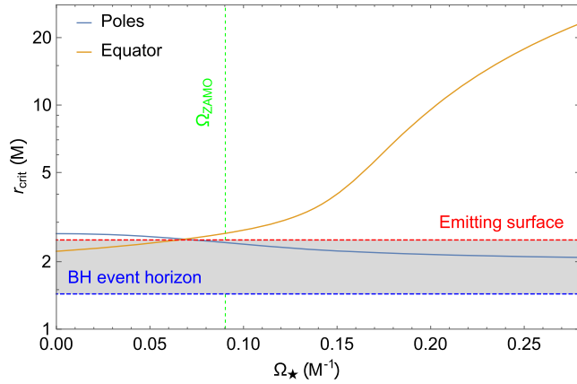
FIG. 11. Critical radius r_{\text{crit}} as a function of the angular velocity of the emitting source \Omega_* at the poles (blue line) and at the equator (orange line). The dashed red line represents the emitting surface and the dashed blue line indicates the BH outer event horizon. The vertical dashed green line is the ZAMO angular velocity \Omega_{\text{ZAMO}} = 0.09M^{-1} . The plot is constructed for a luminosity parameter of A = 0.5 , BH spin of a = 0.9 and radius of the emitting surface of R_* = 2.5M .
