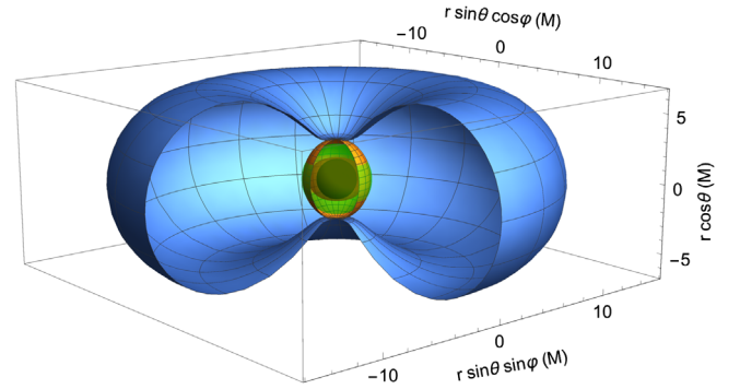
FIG. 12. Critical hypersurfaces for a luminosity parameter of A = 0.5 , BH spin of a = 0.9 and radius of the emitting surface of R_* = 2.5M . The black sphere is the BH outer event horizon with size R_H = 1.44M , the red ellipsoid around the BH outer event horizon represents the ergosphere and the green sphere is the emitting surface. The orange surface is calculated for \Omega_* = 0.05M^{-1} it has r_{\text{crit}}^{\text{eq}} = 2.42M and r_{\text{crit}}^{\text{pole}} = 2.89M . The blue surface is obtained setting \Omega_* = 0.24M^{-1} and has r_{\text{crit}}^{\text{eq}} = 15.65M and r_{\text{crit}}^{\text{pole}} = 2.89M .
