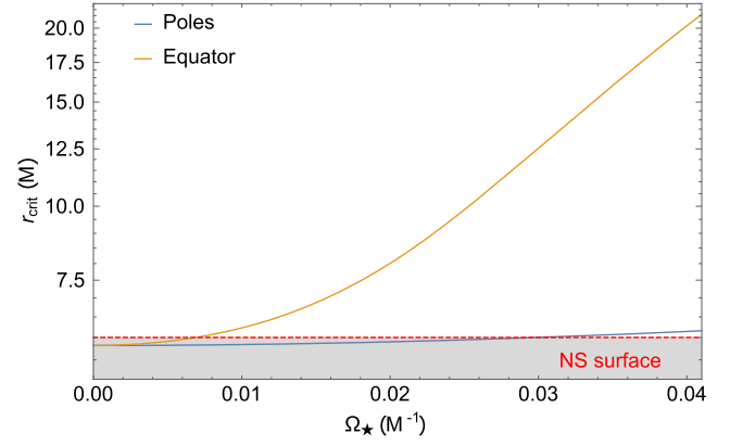
FIG. 5. Critical radius r_{\text{crit}} at the poles (blue line) and at the equator of the NS (orange line) as a function of the NS rotation angular velocity \Omega_{\star} for a luminosity parameter of A = 0.81 . The dashed red line represents the NS surface, the gray area indicates the (nonphysical) solutions inside NS.
