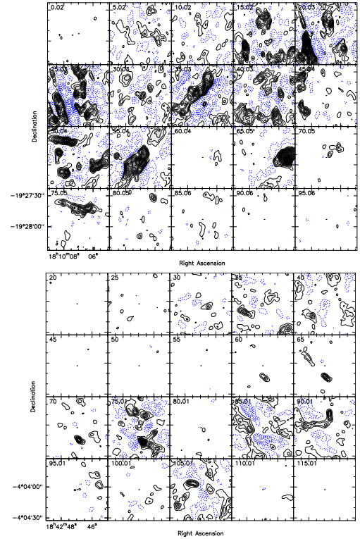
Fig. B.2. CO 2-1 channel maps. These images are the result of averaging the emission over a velocity interval of 5 km/s. The central velocity is labeled on each panel. The contours start at 3\sigma in steps of 3\sigma . No additional uv filtering has been applied to the data. The black circle in each images shows the SMA FOV at 230 GHz.
