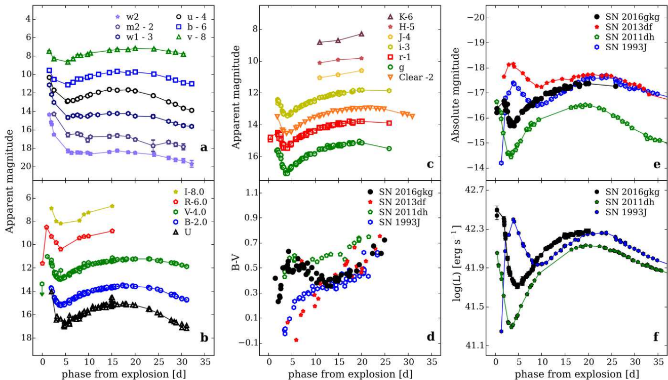
FIG. 1.— (a) UVOT, (b) UBVRI and (c) grizJHK light-curves of SN 2016gkg. (d) B – V color evolution compared with those of SNe 1993J, 2011dh and 2013df. (e) Absolute r light curves compared with those of SNe 1993J ( R -band), 2011dh ( g -band) and 2013df ( R -band). (f) Pseudo-bolometric light curve compared to those of SNe 2011dh and 1993J. The Pseudo-bolometric light curves were computed using Simpson’s rule, integrating the photometric data. At early phase only Vr bands are available. For the missing bands, we assumed constant colors and a 10% uncertainty on the computed flux. Errors for SN 2016gkg were computed assuming a fixed distance modulus ( \mu = 32.11 mag). The data in panels a,b,c,f are available as Data behind the Figure.
