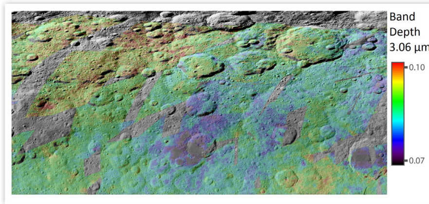
Fig. 4. The band depth at 3.1 \mu\text{m} is indicative of the \text{NH}_4 -phyllsilicates abundance.
