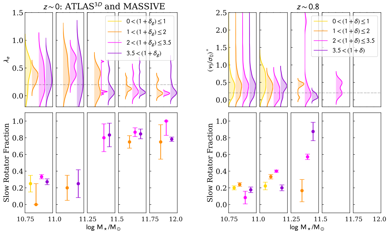
Figure 4. ( Top row: ) The normalized probability distribution functions (PDFs) for \lambda_\epsilon (left, ATLAS ^{3D} and MASSIVE) and (v_5/\sigma_0)^* (right, LEGA-C) for the most massive galaxies in both samples ( \log M_*/M_\odot \geq 10.75 ). The dashed horizontal line shows the slow-rotator threshold (rotational support \leq 0.2 ). ( Bottom row: ) The slow-rotator fractions for ATLAS ^{3D} and MASSIVE (left) and LEGA-C (right). PDFs and points are colored by overdensity. Both LEGA-C and the nearby sample show similar slow-rotator fractions at the lowest masses. However, for galaxies with \log M_*/M_\odot \geq 11.25 , there is a clear separation in the slow-rotator fractions for LEGA-C galaxies while those for the nearby Universe only exhibit a trend with mass.
