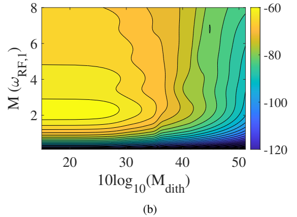
Fig. 6: Simulation of HD_{2\omega_{RF,1}} (a) and HD_{3\omega_{RF,1}} (b) expressed in dB_m obtained varying both M(\omega_{RF,1}) and M_{dith} . See text for details.
