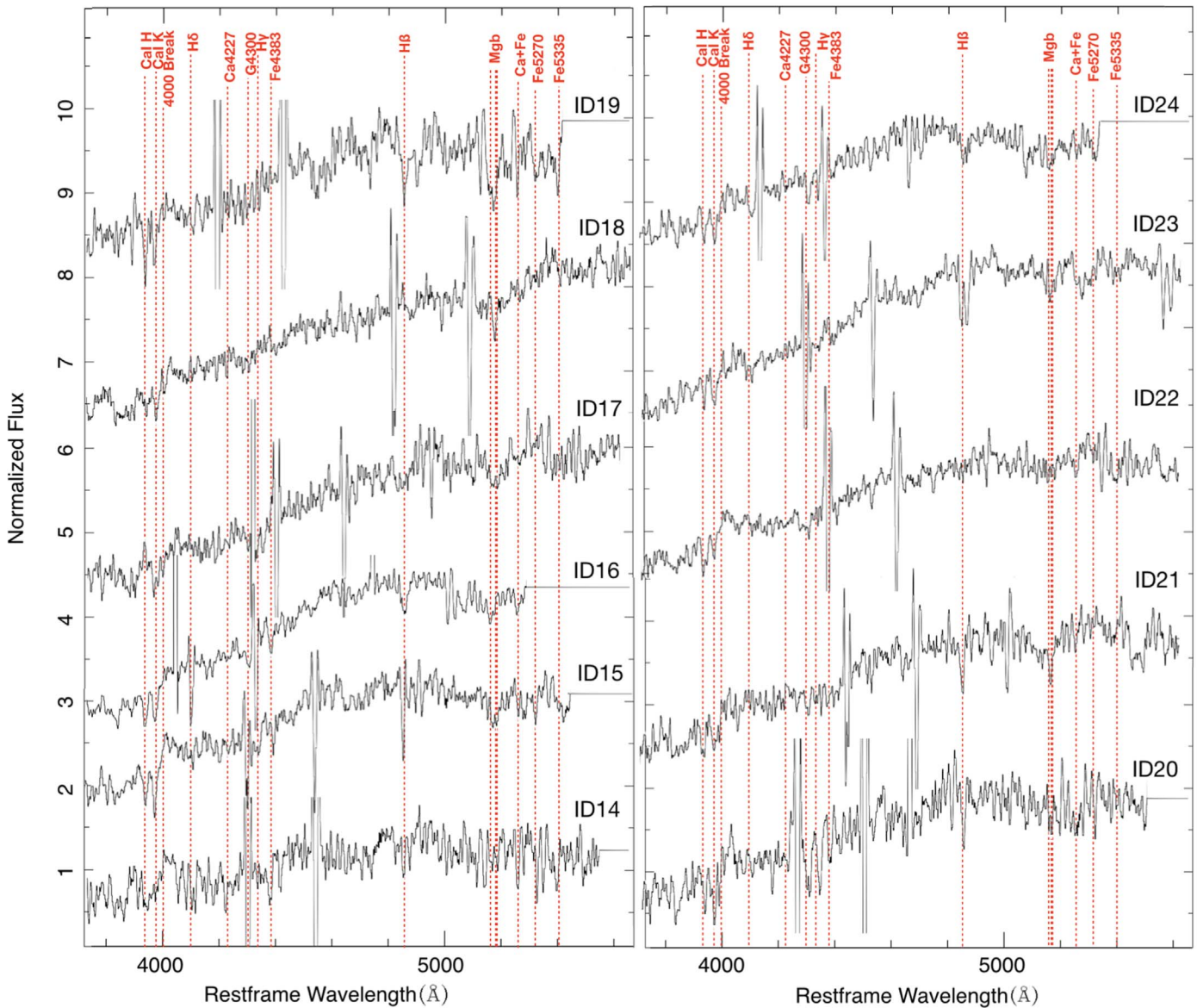
Figure 3. Same as Figure 2, but for the 11 candidates observed in our spectroscopic campaign with TNG (UCMG_TNG_2017), for which we obtain a spectroscopic redshift estimation.
