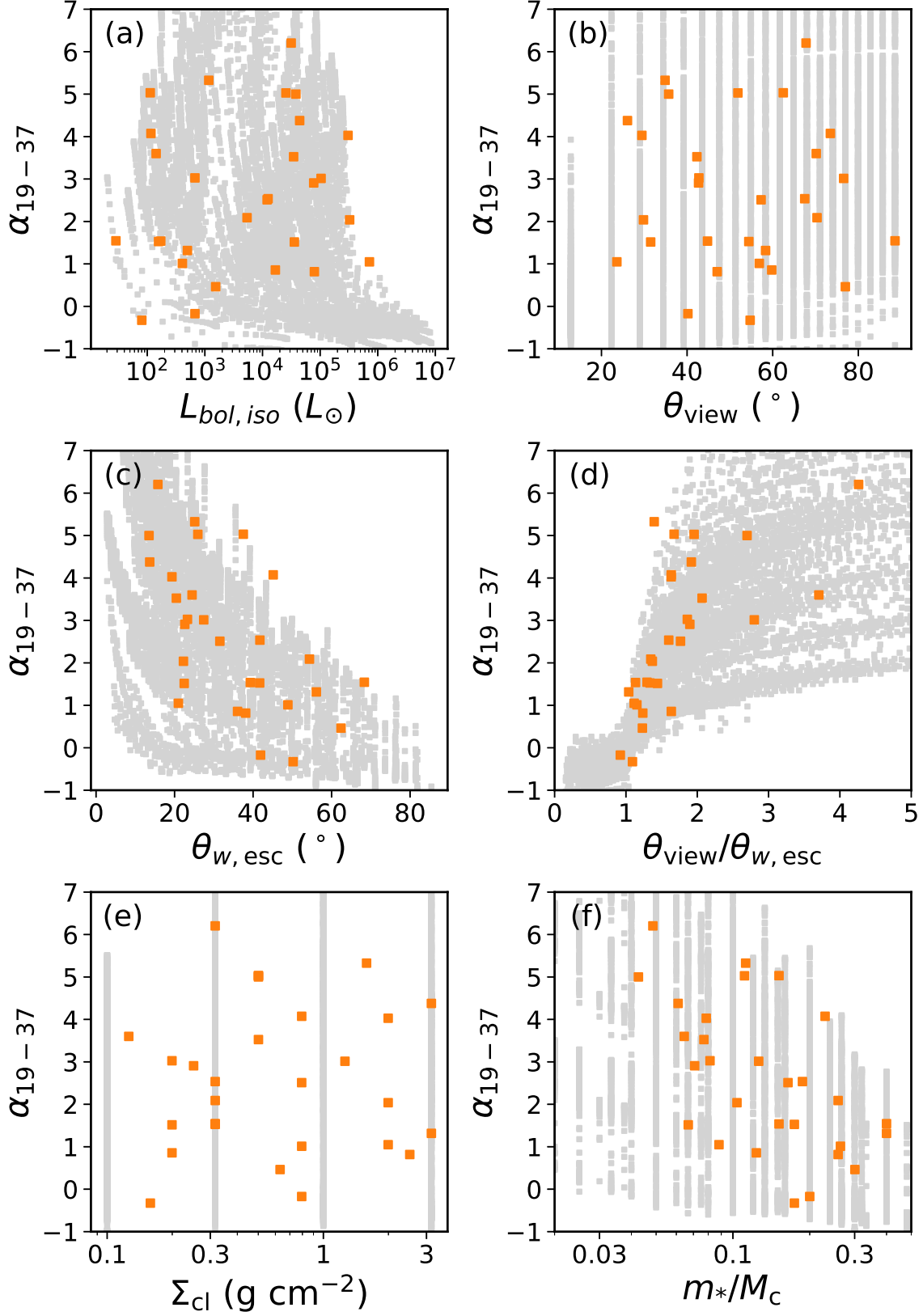
Figure 16. Spectral index, \alpha_{19-37} between 19 \mu\text{m} and 37 \mu\text{m} (see text) versus: the geometric mean isotropic luminosity L_{\text{bol,iso}} (a: top left); the arithmetic mean inclination of viewing angle \theta_{\text{view}} (b: top right); the arithmetic mean opening angle \theta_{w,\text{esc}} (c: middle left); arithmetic mean \theta_{\text{view}}/\theta_{w,\text{esc}} (d: middle right); the geometric mean clump surface density \Sigma_{\text{cl}} (e: bottom left); and geometric mean m_*/M_c (f: bottom right) returned by the best five or fewer models with R_c \lesssim 2R_{\text{ap}} and \chi^2 < \chi_{\text{min}}^2 + 5 . The grey squares represents the ZT18 protostar models. Note that the spectral index of the models are calculated without foreground extinction and thus could be different from observations.
