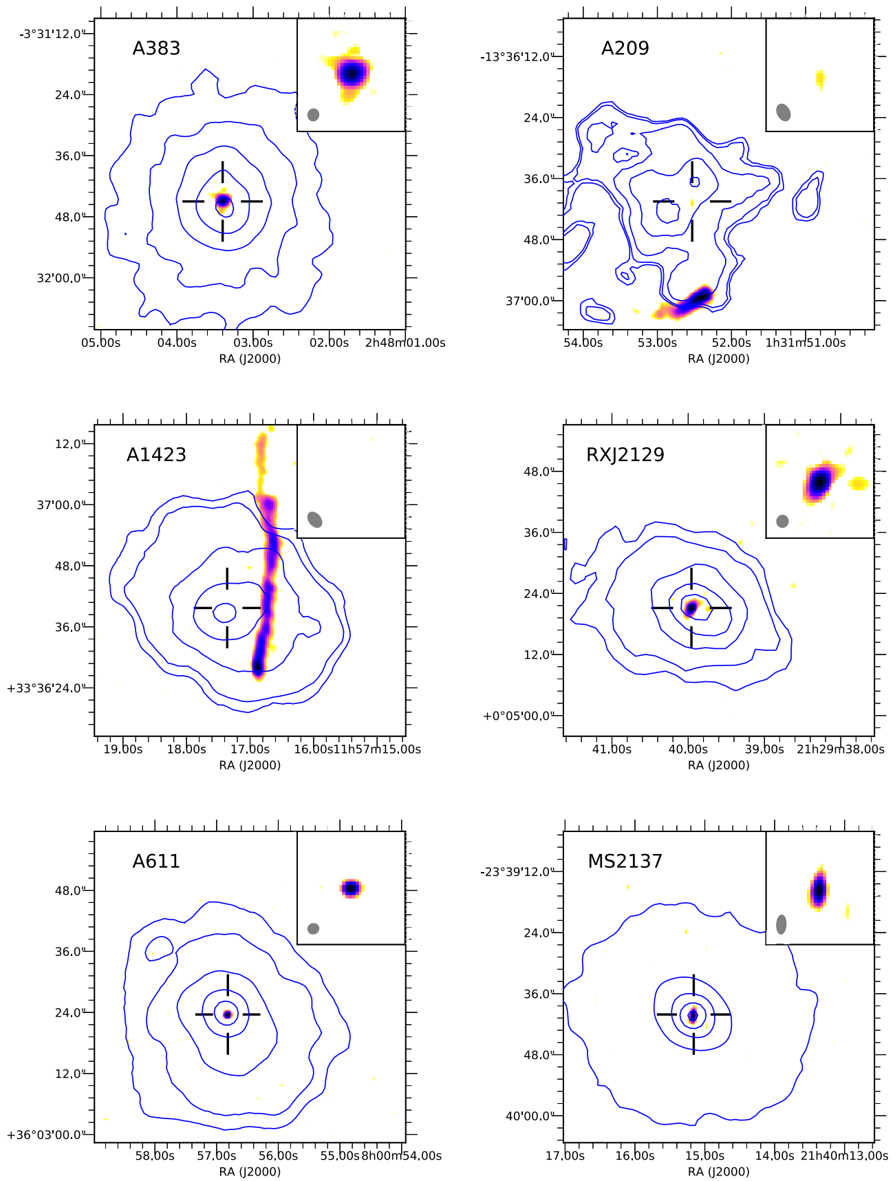
Figure 1. Radio images overlapped with the Chandra contours (blue lines). Central crosses indicate the position of the BCG obtained from the HST optical image. The FOV is 1' \times 1' . The small panel in the top right corner shows the enlarged central region with a FOV 10'' across. The beam size is shown as a gray ellipse in the bottom left corner. The color scale ranges from 3\sigma to the maximum flux in each field with a logarithmic step. These images are generated with APLpy (Robitaille & Bressert 2012).
