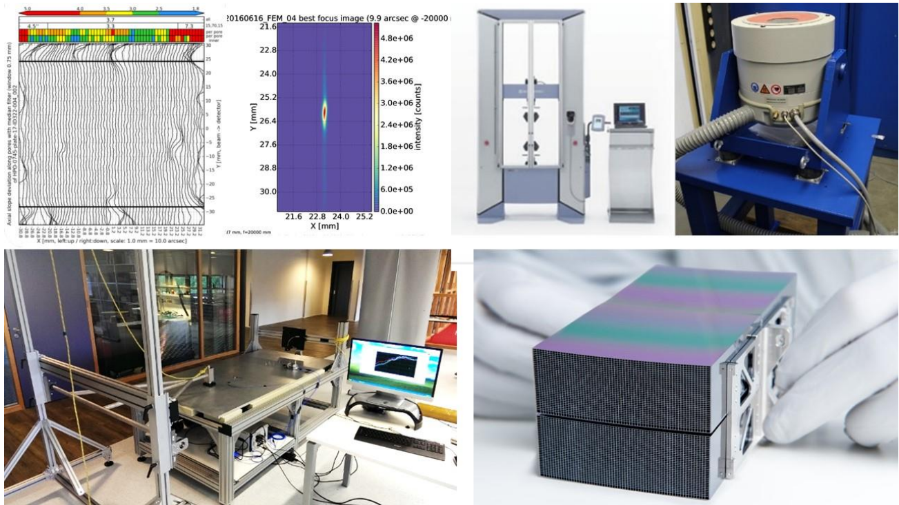
Figure 8: The production of the SPO MM is accompanied with extensive metrology, starting with component level and part inspection tests, and finishing with X-ray performance characterisations. Top left shows the topogramme measured with the on-line fringe reflection metrology system installed on each of the stacking robots, centre left shows the PSF of a MM measured at XPBF. Top centre right: automatic pulling station for component tests, top right: shaker, bottom left shock table, bottom right: completed MM.
