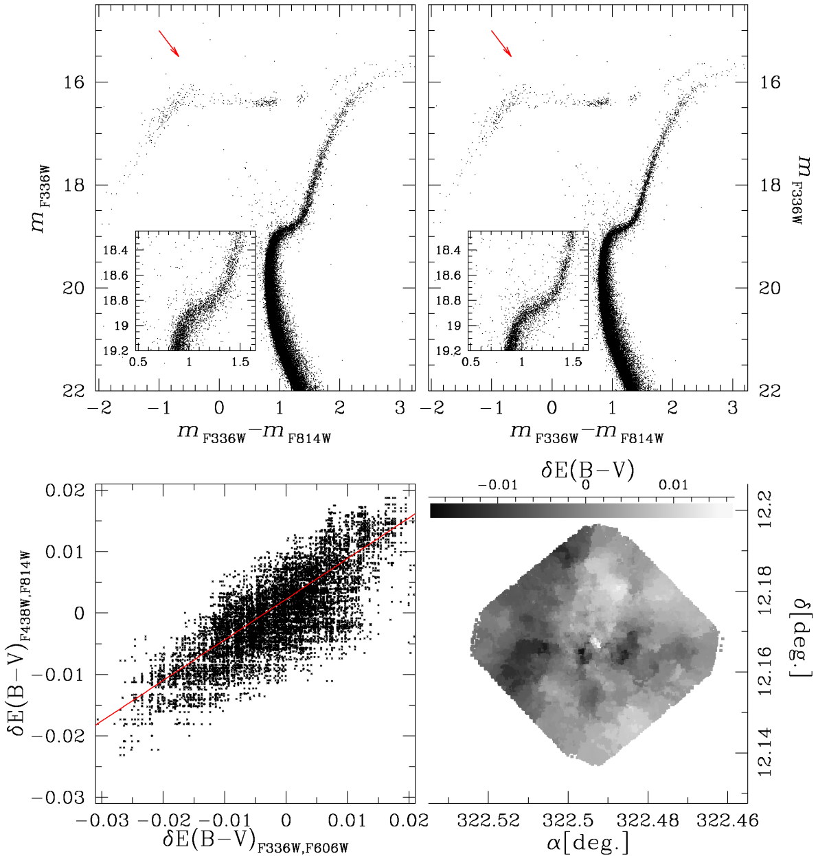
Figure 3. Top panels show the m_{\text{F336W}} versus m_{\text{F336W}} - m_{\text{F814W}} CMDs before (left panel) and after (right panel) the differential reddening correction; the red arrow is the reddening vector. The insets show a zoom-in around the SGB region. Bottom left panel shows a comparison between the values of differential reddening inferred from m_{\text{F606W}} versus m_{\text{F336W}} - m_{\text{F606W}} and m_{\text{F814W}} versus m_{\text{F438W}} - m_{\text{F814W}} CMDs. The red line is obtained from a least-squares fit of the \delta E(B-V)_{\text{F336W,F606W}} and \delta E(B-V)_{\text{F438W,F814W}} . Bottom right panel presents the map of the differential reddening.
