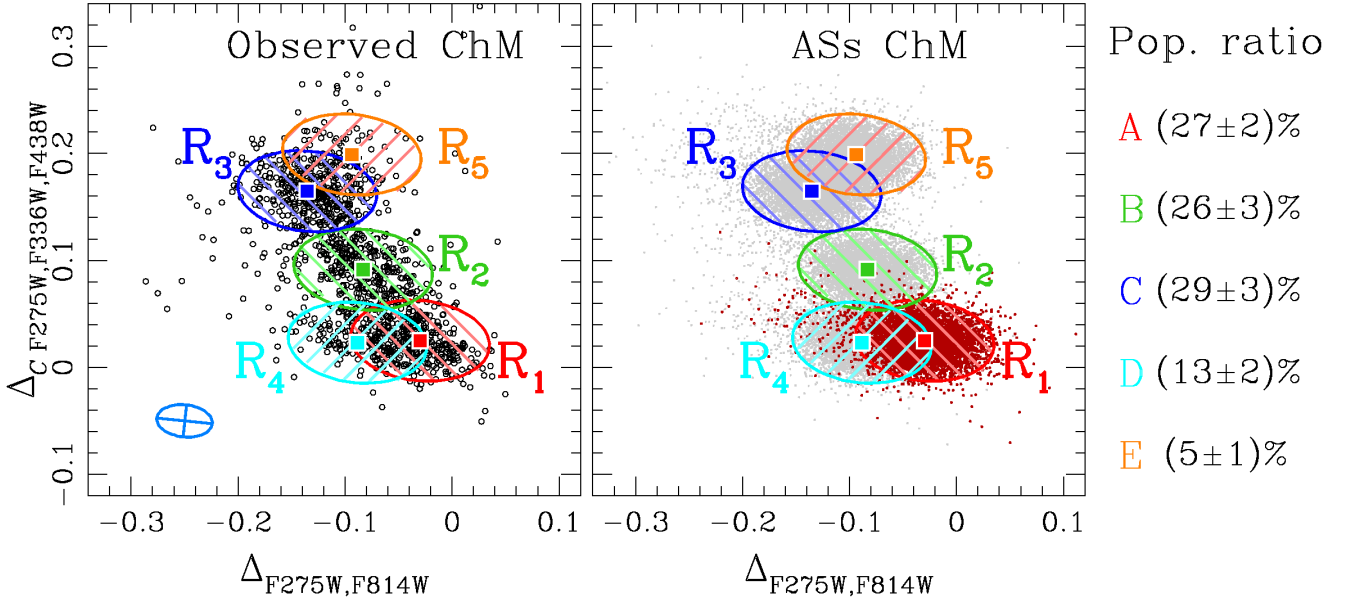
Figure 12. Procedure adopted to estimate the fraction of stars in each population. Left panel shows the observed \Delta_{CF275W,F336W,F438W} versus \Delta_{F275W,F814W} ChM (black empty circles). The azure ellipse is indicative of the dispersion of a single population ( \sigma_{\text{obs}} ). The regions R_i correspond to a size of 2.5 \times \sigma_{\text{obs}} . Coloured squares correspond to the centre of the identified populations. Right panel shows the ASs \Delta_{CF275W,F336W,F438W} versus \Delta_{F275W,F814W} ChM. The regions R_i have the same size and are located in the same positions of the regions of the left panel.
