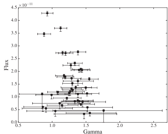
Figure 5. Time-resolved analysis of flux and photon index through observations 2 and 3. Each data point is derived from a 1000s subsection of data.
