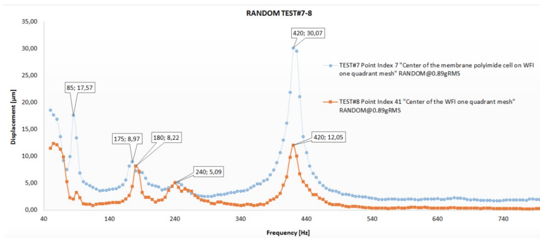
Figure 11. WFI OBF filter – Spectrograms of two points at the centre of one quadrant, obtained by low level random vibration test (0.89 g RMS). Red curve refers to a point on the metallic mesh, while blue curve is relevant to a point at the centre of one cell. Lowest frequencies confirm quite well numerical results (91 Hz and 180 Hz for the mesh). The 420 Hz peak is due to the mechanical jig used to mount the filter.
