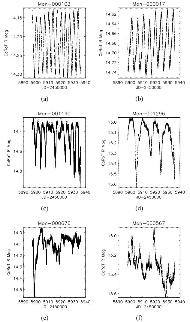
Fig. 3. CoRoT light curves of CTTSs from 2011 showing different photometric variabilities. Panels a) and b) correspond to spot-like light curves, c) and d) to AA Tau-like light curves, e) is a non-periodic light curve caused by obscuration by circumstellar material, and f) is a non-periodic light curve dominated by accretion bursts. The light-curve magnitude was calibrated using the R filter with a zero point of 26.74 mag, as described in Cody et al. (2014) .
