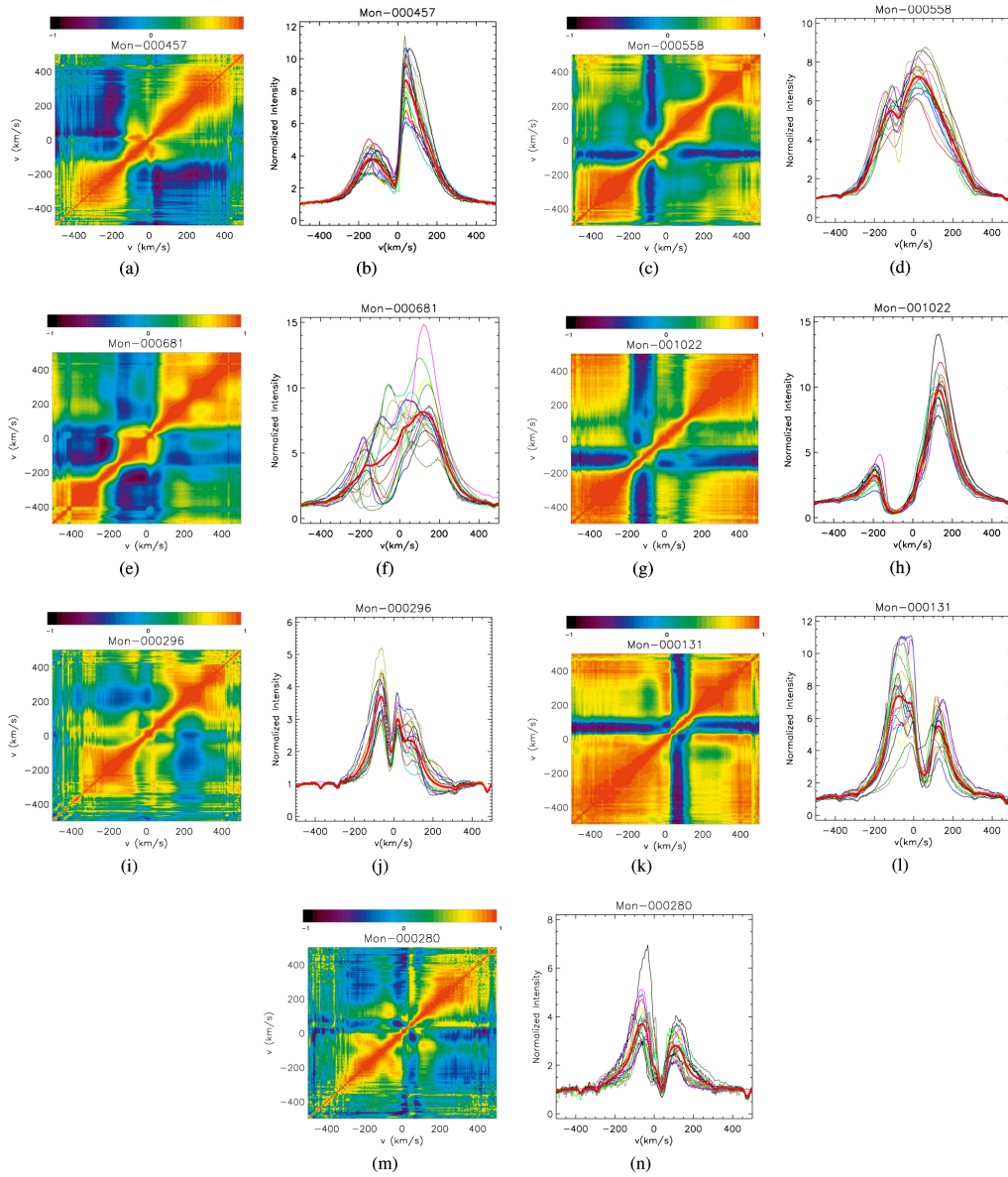
Fig. A.1. Correlation matrices ( left ) of the H \alpha line of selected CTTSs and the corresponding line profiles ( right ). In the left panels , the color range corresponds to the value of the linear correlation coefficient, r(i, j) , between different velocity bins ( i and j ), of the H \alpha line profiles, as described in Sect. 11. Perfect anticorrelation corresponds to -1 (black), no correlation to 0 (light blue), and a perfect correlation to 1 (orange). When i = j , r(i, j) = 1 , and for all values of i and j , r(i, j) = r(j, i) , implying that the matrix is symmetrical relative to the diagonal. In the right panels , different colors correspond to spectra observed in different nights, and the thick red line is the average line profile. The stars in this group present anticorrelation of some part of the line profile. The anticorrelation seen in these stars is associated with blue- or redshifted absorption or emission that varies in antiphase with the rest of the profile. For example, when in panel a (Mon-000457) the red wing emission increases in intensity, the blue wing emission decreases.
