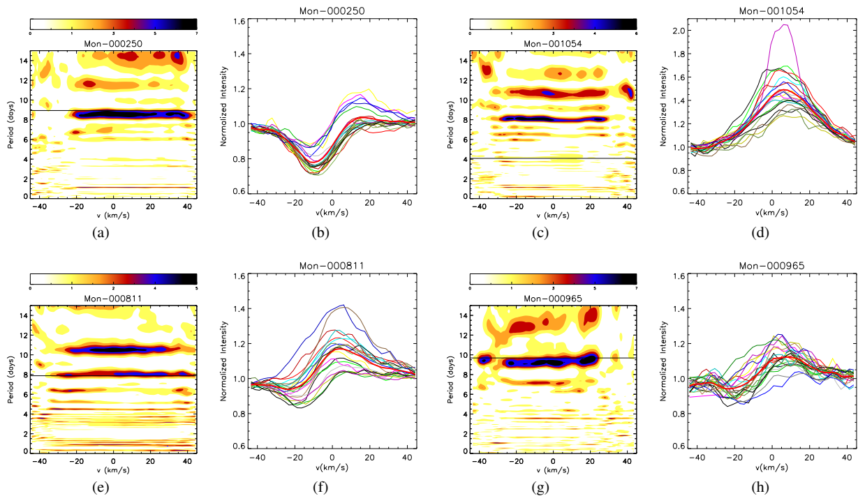
Fig. 17. Periodic stars in the He I 6678 Å that also showed a periodicity in the CoRoT light curves. Bidimensional periodograms of the He I line ( first and third columns ). The color code represents the power of the periodogram, varying from zero (white) to the maximum power intensity (black). The black horizontal lines correspond to the period of the 2011 CoRoT light curve. The second and fourth columns present the He I 6678 Å lines used to calculate the periodograms. Different colors correspond to different nights of observation, and the thick red line is the average line profile.
