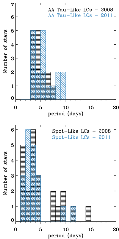
Fig. 6. Period distribution of the CTTs observed in 2008 (black) and 2011 (blue). Top: AA Tau-like light curves. Bottom: spot-like light curves. AA Tau-like stars clearly present periods within the range of spot-like systems.
