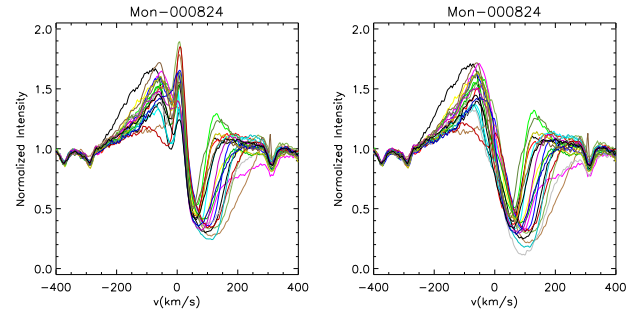
Fig. 1. H \alpha emission lines of a CTTS before ( left ) and after ( right ) sky subtraction that show the removal of the nebular emission contribution. The nebular component is the very sharp, narrow emission seen near the line center in the left panel. Different colors correspond to different observing nights.
