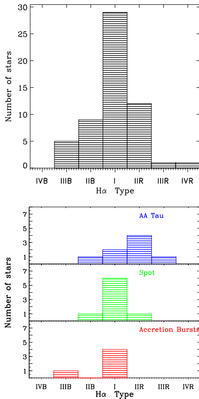
Fig. 12. Distribution of H \alpha profile types according to the classification of Reipurth et al. (1996). Top : all the CTTs observed with FLAMES. Bottom : CTTs observed both with FLAMES and CoRoT. Light curves classified as spot-like, AA Tau-like, and accretion burst are shown as a function of profile type.
