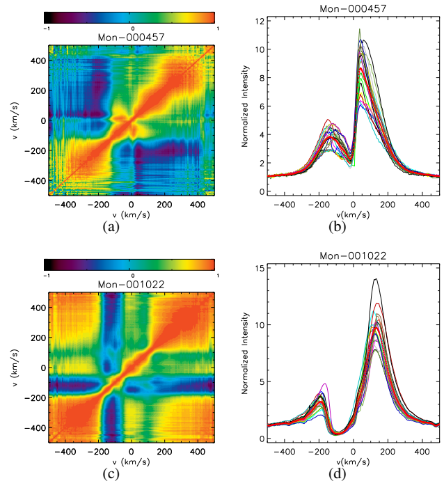
Fig. 21. Examples of correlation matrices ( left ) of the H\alpha line of two CTTs and the corresponding line profiles ( right ). In panels a ) and c ), the color range corresponds to the value of the linear correlation coefficient between the different velocity bins of the H\alpha line profiles. Perfect anticorrelation corresponds to -1 (black), no correlation to 0 (light blue), and a perfect correlation to 1 (orange). In panels b ) and d ), different colors correspond to spectra observed in different nights, and the thick red line is the average line profile. The correlation matrices and H\alpha line profiles of all the CTTs in our sample observed with FLAMES are presented in the Appendix.
