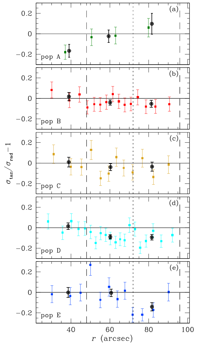
Figure 4. Deviation from tangential-to-radial isotropy (horizontal line) for the five populations (color-coded as in Figure 1). Vertical lines mark the locations of r_h , 1.5 \times r_h , and 2 \times r_h .
