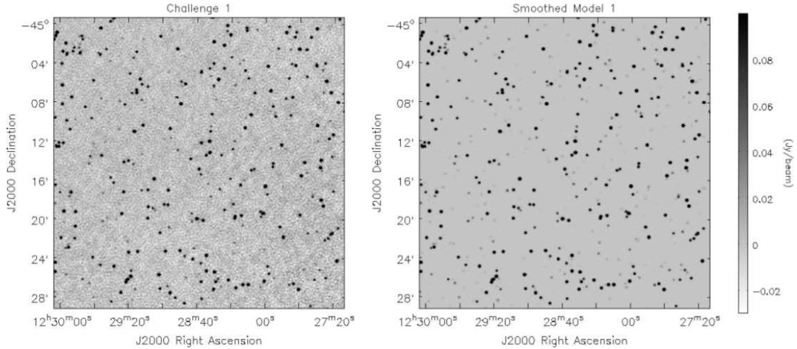
Figure 1. A subsection of the first Data Challenge image (left), and the input source distribution to this image (right). This image includes sources distributed randomly with a flux density distribution that is uniform in the logarithm of flux density. This distribution gives rise to a much higher surface density of bright sources, and proportionally more bright sources compared to faint sources, than in the real sky.
