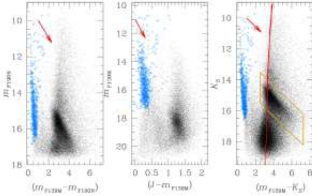
Figure 7. CMDs based on the WFC3/IR data. Left-hand panel: m_{F139M} versus (m_{F139M} - m_{F190N}) CMD. Middle panel: m_{F139M} versus (J - m_{F139M}) CMD. Right-hand panel: K_S versus (m_{F139M} - K_S) CMD. Blue open circles depict stars in common with the Gaia -DR2 catalogue. In each CMD, the direction of the reddening vector is indicated by a red arrow. The reddening vector is computed by assuming an arbitrary extinction A_{F139M} in each plot and the extinction index \alpha = 2.3 of Nogueras-Lara et al. (2018). A PARSEC isochrone for 10-Gyr-old stars with [\text{Fe}/\text{H}] = -0.16 at 8.2 kpc from the Sun representing the Bulge population is fitted by eye as reference in the rightmost panel. The gold rectangle marks the location of the Bulge red clump.
