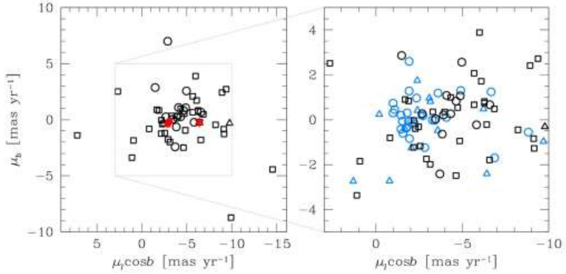
Figure 24. VPDs of the candidate MSs (black points). The red asterisk marks the PM of Sgr A*, while the two red points indicate the PMs of the Arches and Quintuplet clusters. As in Fig. 14, circles, squares, and triangles represent MSs in the Primary, Secondary, and Other samples, respectively. The right-hand panel is a zoomed-in view of the left-hand panel, in which we also plot in blue the confirmed MSs in our field, as a reference.
